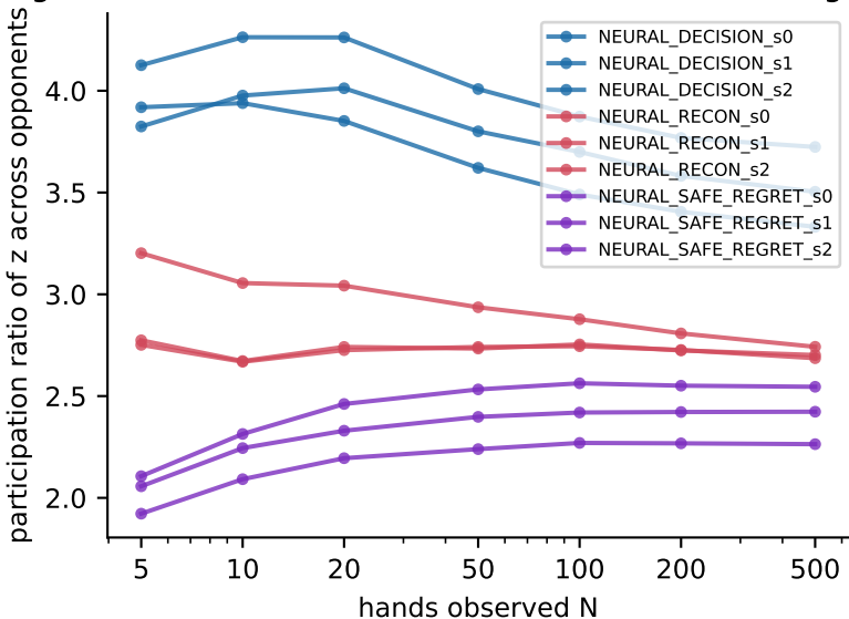
Figure 8: effective latent dimension vs N (linear diagnostic)
