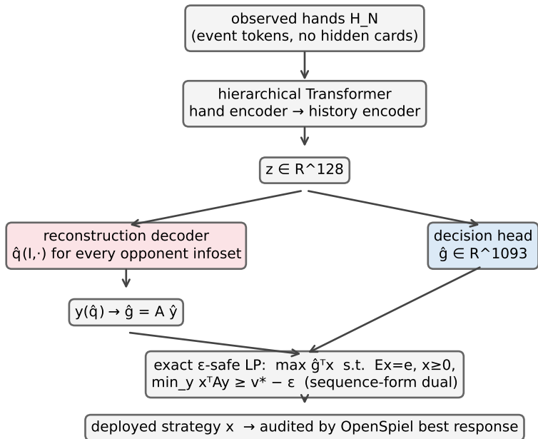
Figure 9: two objectives, one safe solver
