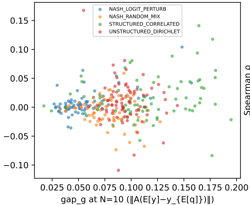
(a) per-opponent gap vs advantage, \rho=0.15
