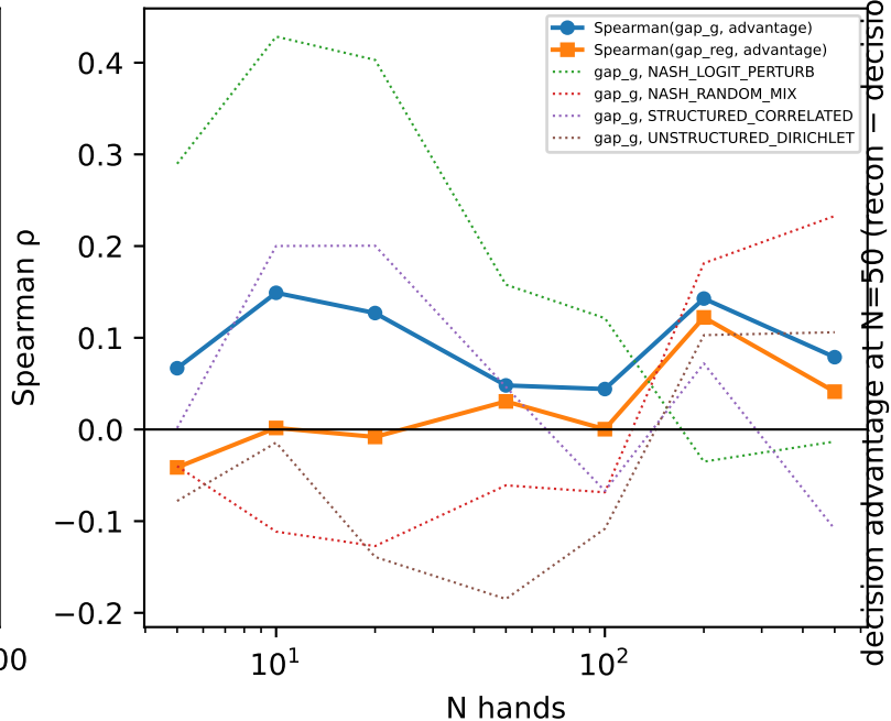
(b) correlation vs N
