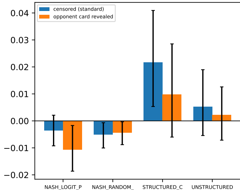
(c) censoring toggle, 3000-step matched 133k/131k models
