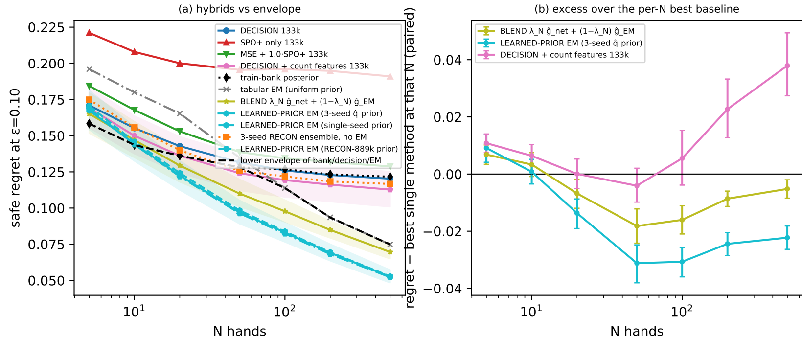
Figure V3-T5: empirical-Bayes hybrids
