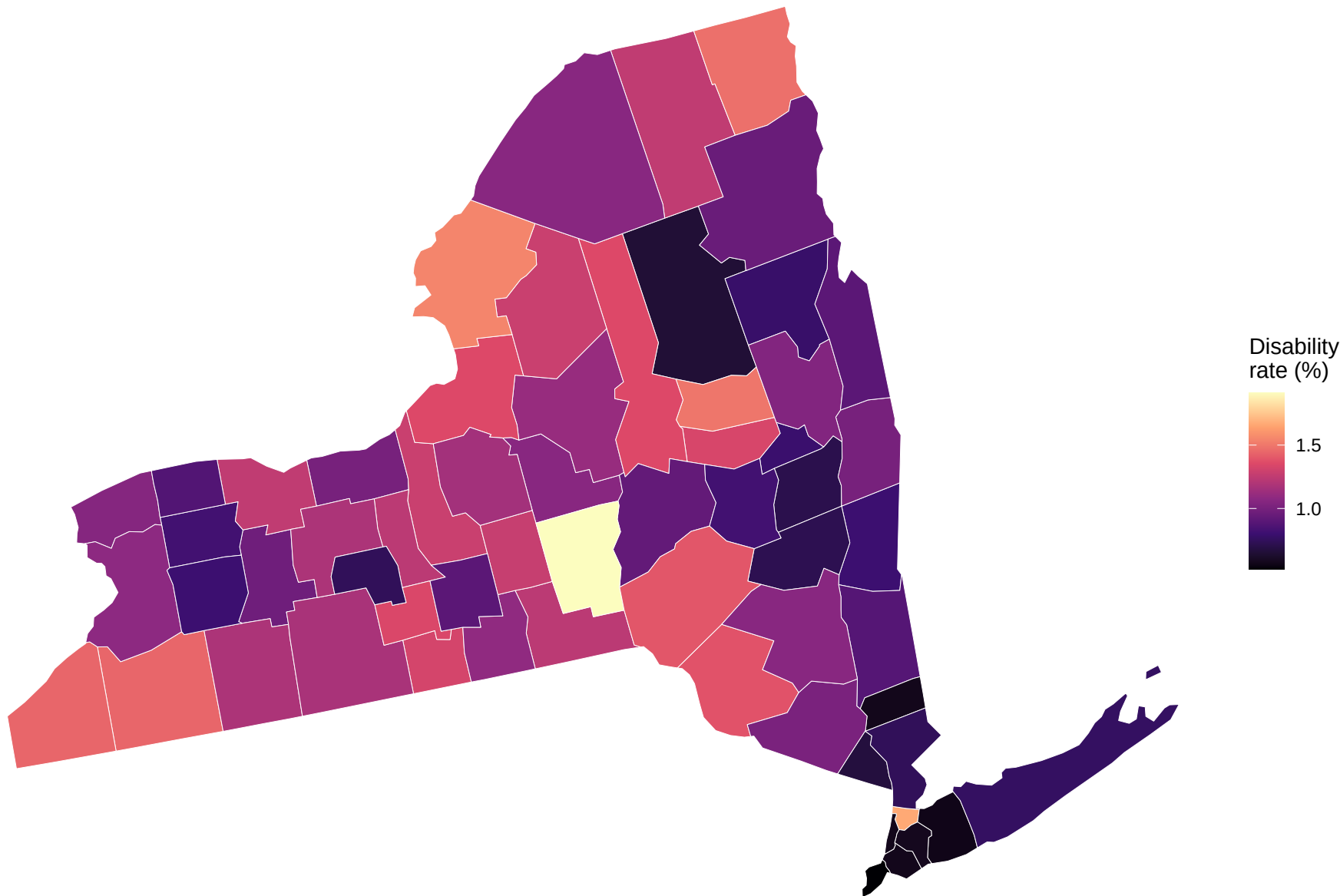
Disability Rate by County, New York (2022)
