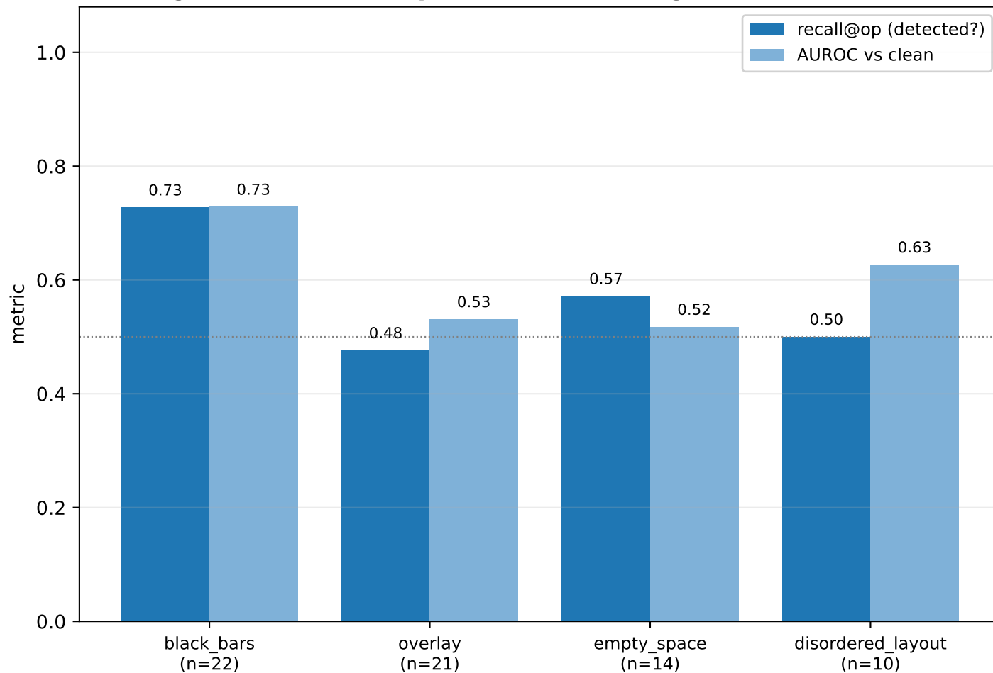
Stage 1 — DETECTION per class (does the gate catch the error?)
