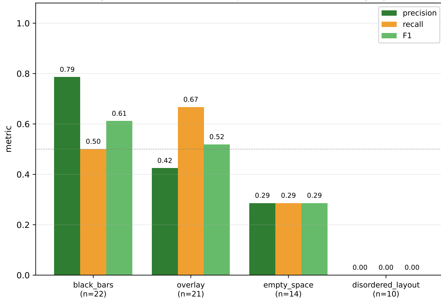
Stage 2 — CLASSIFICATION per class (correct category?)
