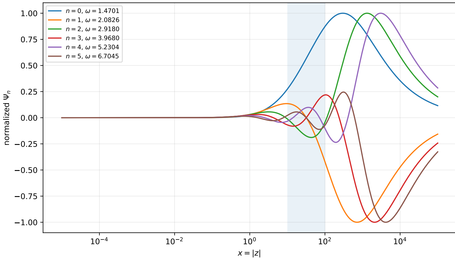
Full Heun eigenfunctions from Frobenius--Frobenius shooting, t = 1000
