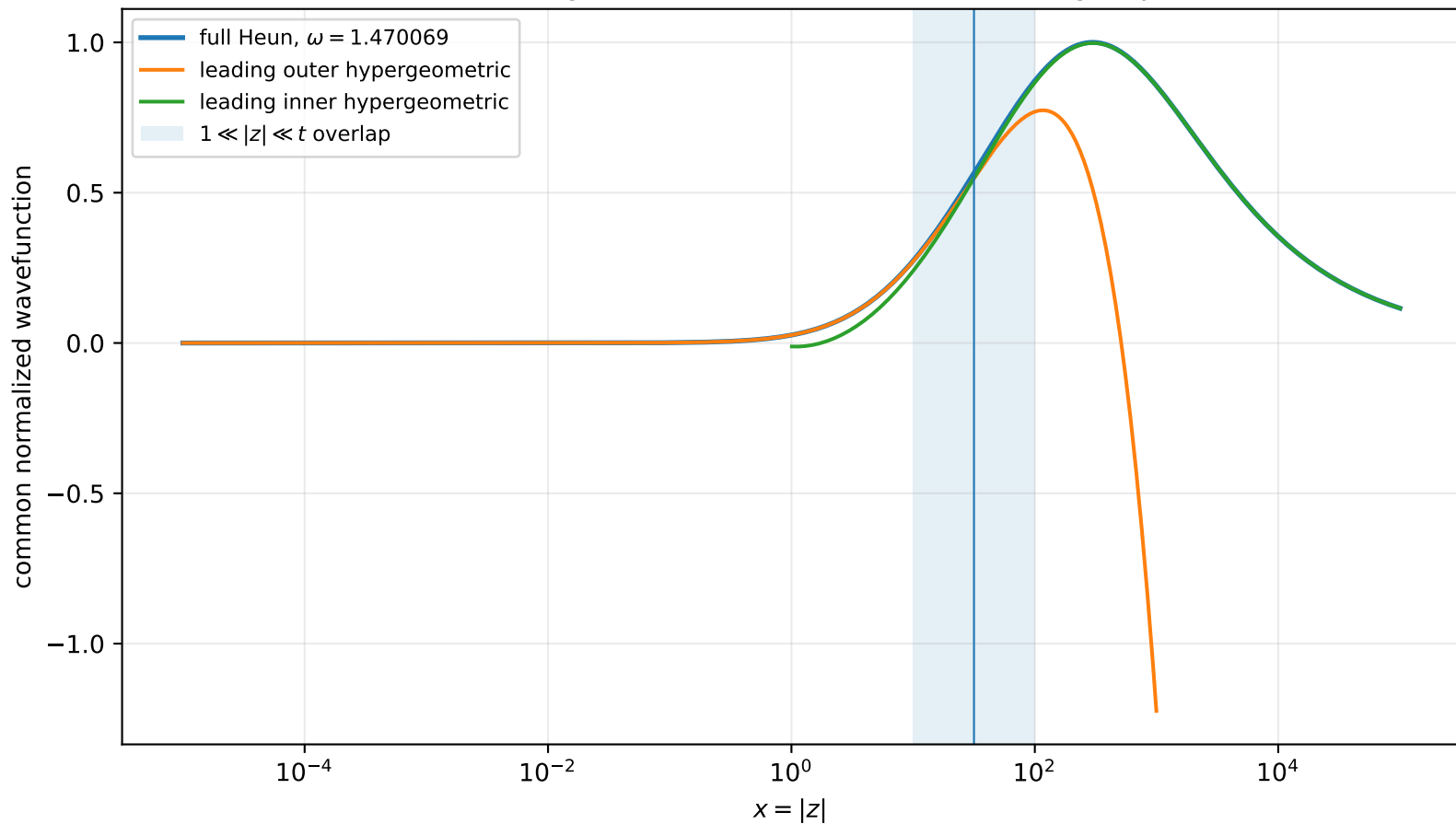
One full Heun eigenmode resolved into the two large- t patches
