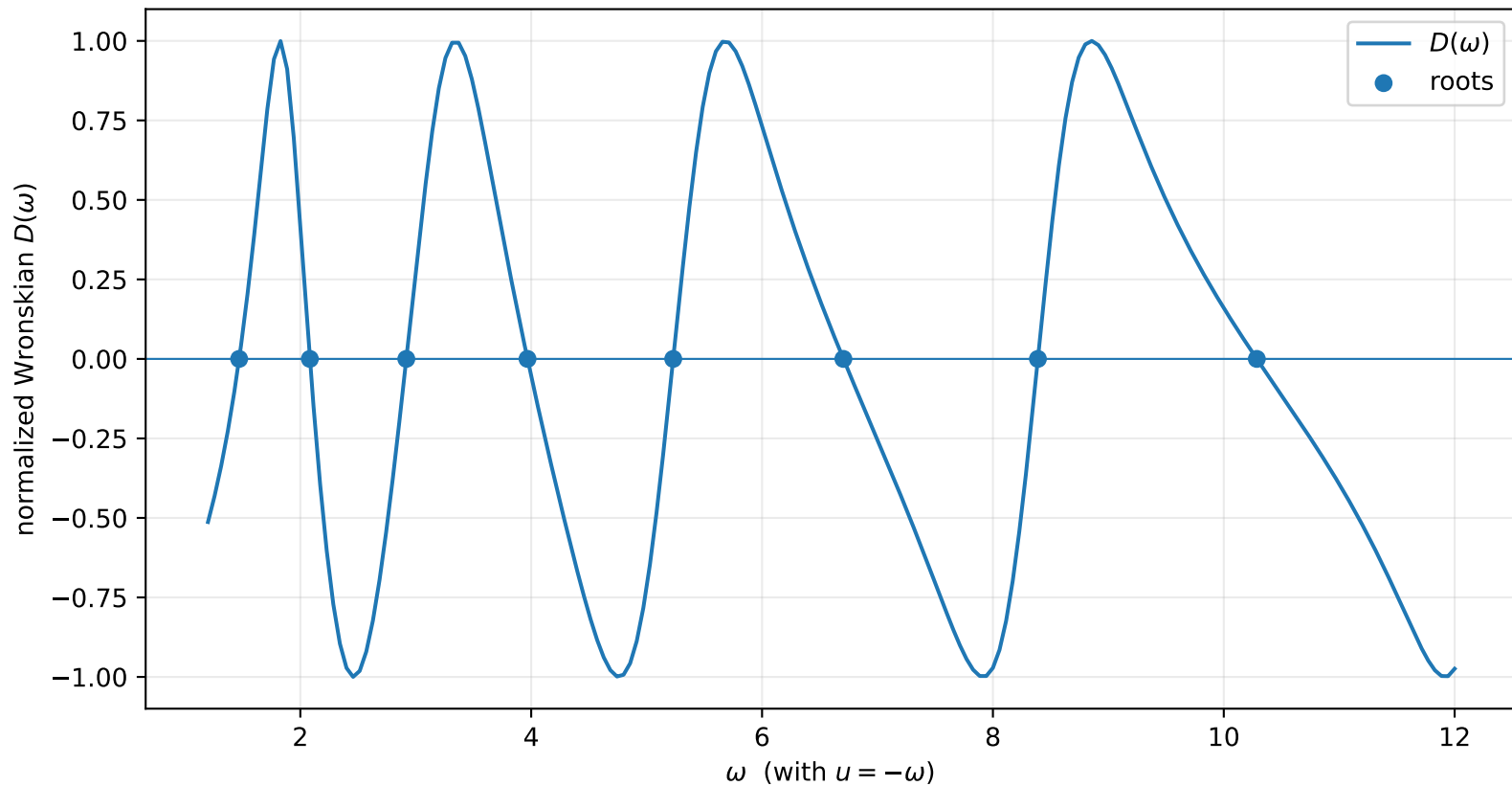
Full Heun shooting spectrum, t = 1000
