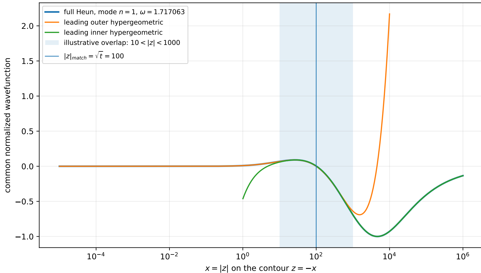
Mode matching for the full Heun eigenmode at t = 10000
