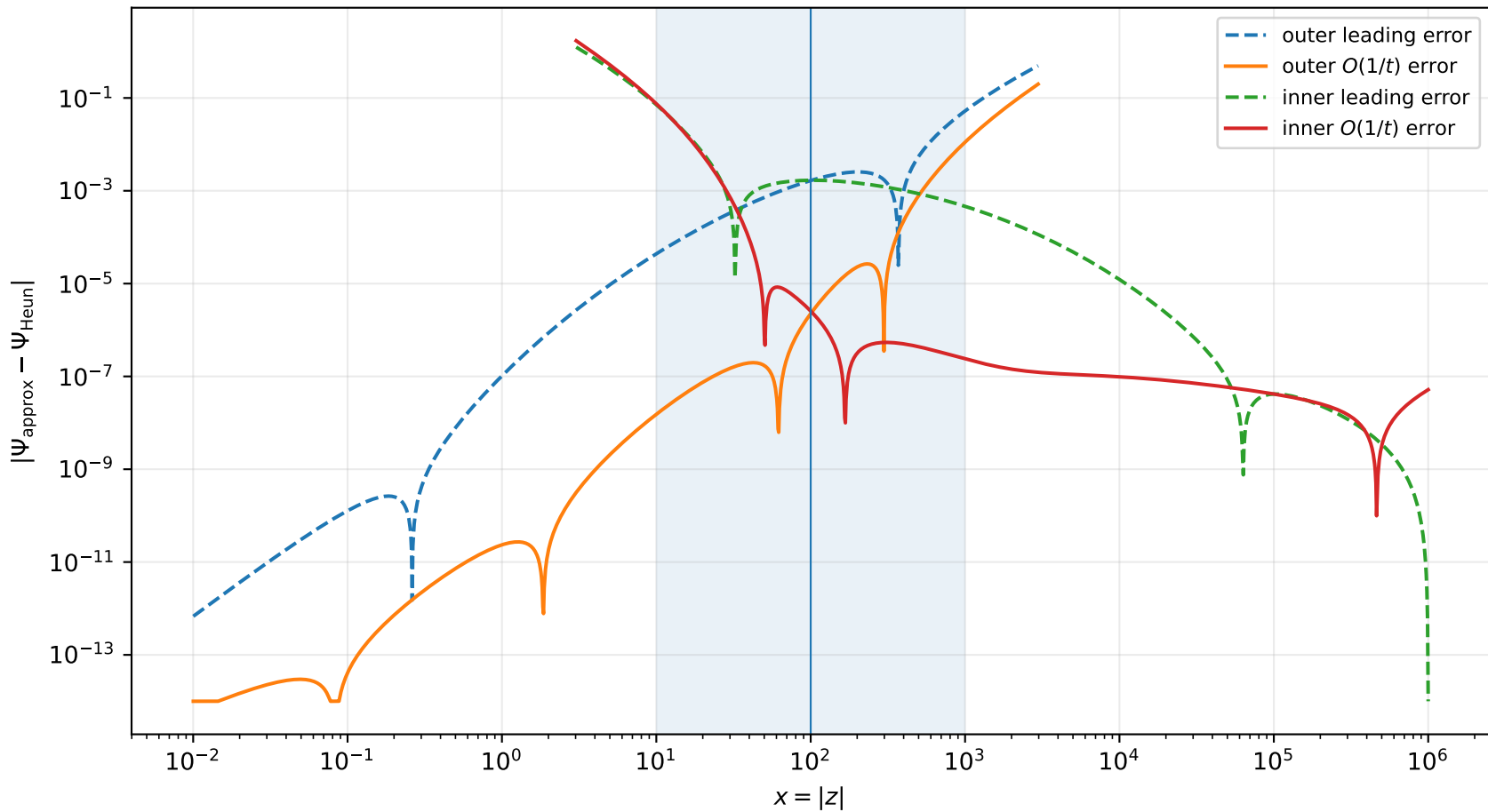
Does the first diffeomorphism correction improve the wavefunction?
