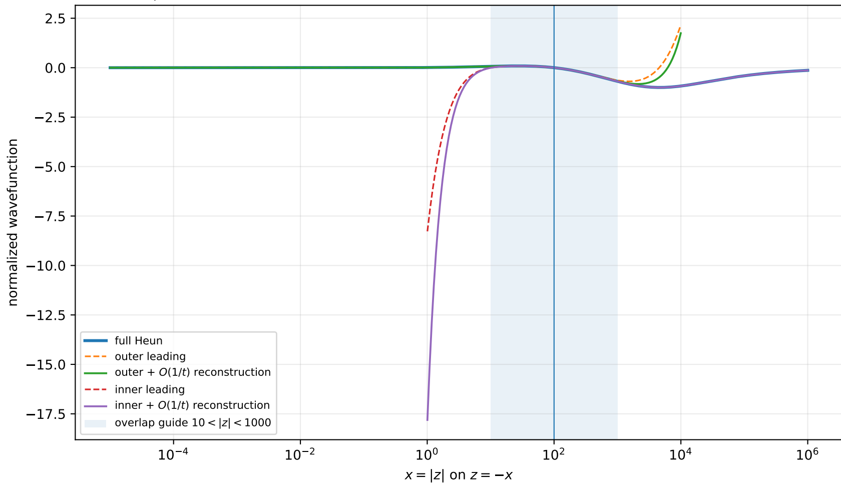
Paper-consistent first wave-function correction, t = 10000 , n = 1 , \kappa^2 = -0.556875
