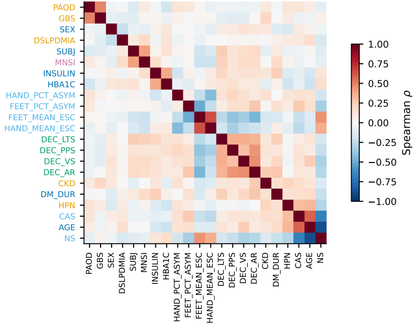
a Correlation structure (clustered)
