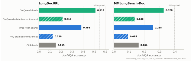
Figure 2: Two observations from the page-level system, per cell: (i) ColQwen2-fresh outperforms the page-level attention router (a loss of roughly 10 points for the router); (ii) both scorers collapse when committed once, so reversibility is a general property of the multi-query regime rather than being scorer-specific.
