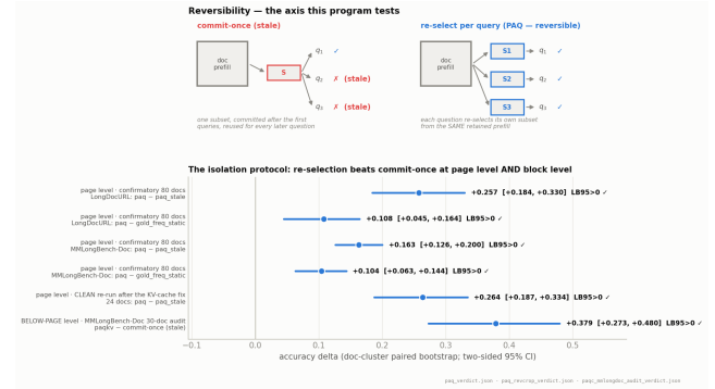
Figure 3: Reversibility, the tested axis. Top: a commit-once deployment reuses one subset for every question and goes stale; re-selection re-derives the subset per query from the same retained prefill. Bottom: the isolation protocol across granularities: the confirmatory page-level contrasts, the clean re-run after the cache fix, and the block-level PAQ-KV contrast. Every interval excludes zero.
