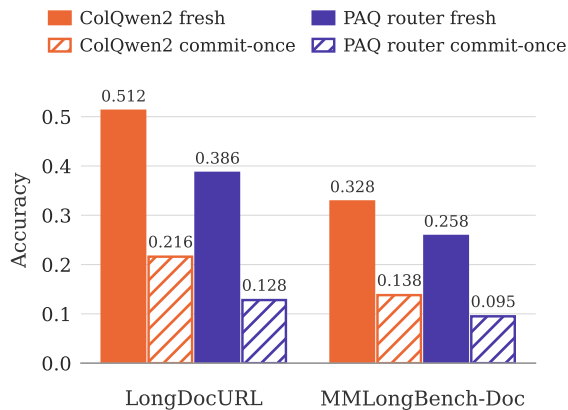
Figure 6: Two observations from the page-level system, per cell (solid bars = per-query fresh selection, hatched open bars = the same scorer committed once): (i) ColQwen2-fresh outperforms the page-level attention router (a loss of roughly 10 points for the router); (ii) both scorers collapse when committed once, so reversibility is a general property of the multi-query regime rather than being scorer-specific. PAQ here is the earlier page-level router of this appendix, not PAQ-KV; the below-page PAQ-KV comparison at matched budget is in Table 1. Historical cohort, uncorrected ColQwen2 loader (disclosed above).
