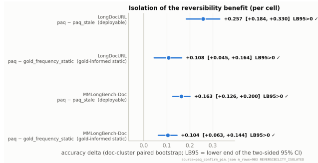
Figure 5: Per-cell forest of the two page-level isolation contrasts at b = 5\% . Intervals are document-clustered two-sided 95% CIs; all four exclude zero.
