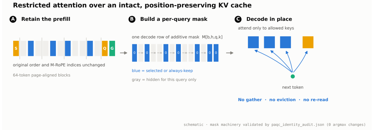
Figure 2: Restricted-attention mechanism. A: The retained cache keeps scaffold, page content in 64-token page-aligned blocks, question, and generated tokens at their original positions. B: For each decode row, the 4D additive mask exposes only selected blocks and the always-keep set; masked blocks remain available to later questions. C: Decode attends to that view without gathering or evicting K/V, so M-RoPE indices remain untouched. An all-true mask reproduced native decode in every audited case (zero mask-specific argmax changes).
