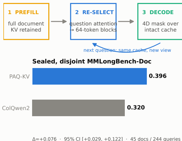
Figure 1: Method and sealed result at a glance. On fresh, disjoint MMLongBench-Doc, PAQ-KV@5% scores 0.396 versus 0.320 for corrected-loader ColQwen2 ( +0.076 , document-clustered 95% CI [+0.029, +0.122] ; 45 documents, 244/244 queries).
