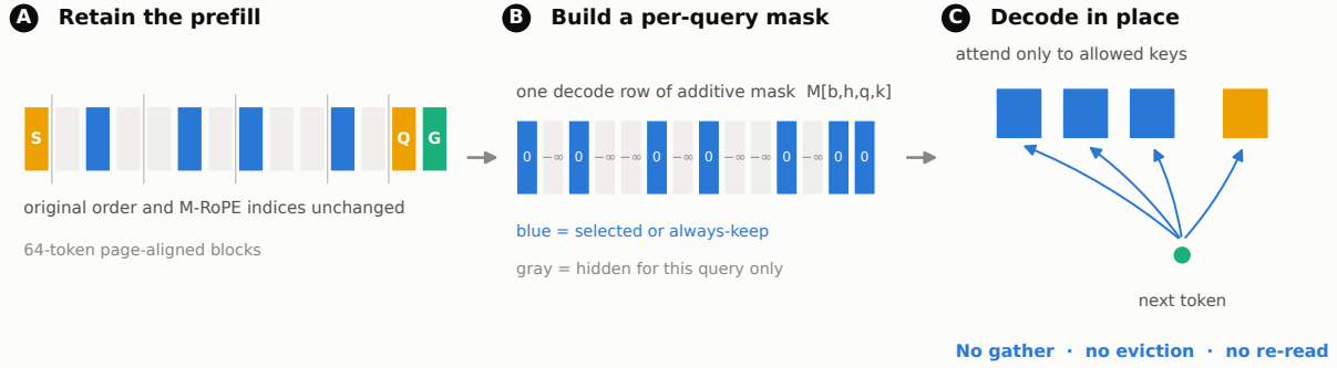
Figure 2: Restricted-attention mechanism. A : The retained cache keeps scaffold, page content in 64-token page-aligned blocks, question, and generated tokens at their original positions. B : For each decode row, the 4D additive mask exposes only selected blocks and the always-keep set; masked blocks remain available to later questions. C : Decode attends to that view without gathering or evicting K/V, so M-RoPE indices remain untouched. An all-true mask reproduced native decode in every audited case (zero mask-specific argmax changes).
