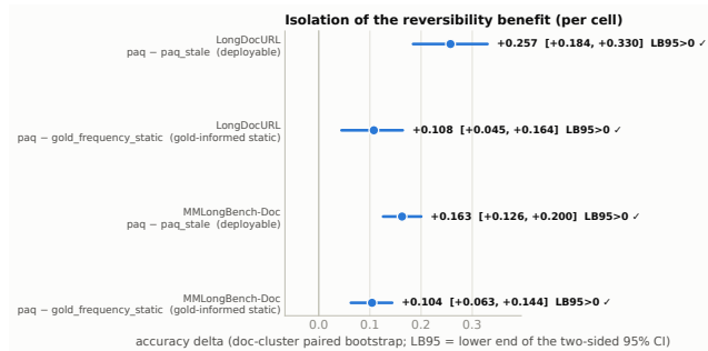
Figure 5: Per-cell forest of the two page-level isolation contrasts at b = 5\% . Intervals are document-clustered two-sided 95% CIs; all four exclude zero.
