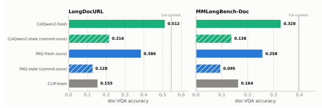
Figure 3: Two observations from the page-level system, per cell: (i) ColQwen2-fresh outperforms the page-level attention router (a loss of roughly 10 points for the router); (ii) both scorers collapse when committed once, so reversibility is a general property of the multi-query regime rather than being scorer-specific.
