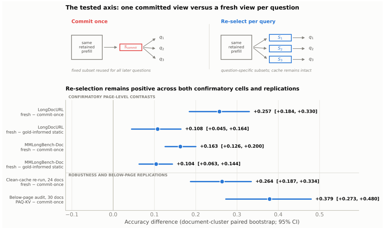
Figure 4: Reversibility, the tested axis. Top: commit-once reuses one fixed subset across questions, whereas re-selection derives a question-specific view from the same intact prefill. Bottom: document-clustered two-sided 95% intervals for the confirmatory page-level contrasts, the clean-cache re-run, and the below-page PAQ-KV replication. Every interval excludes zero.
