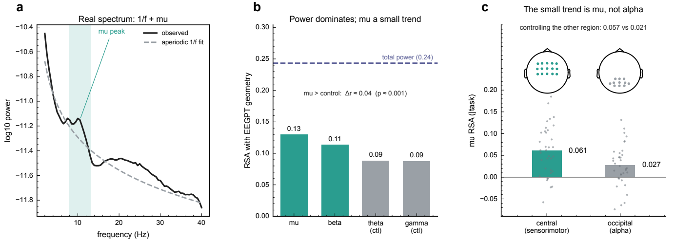
Fig. 1. Auditing EEGPT on motor imagery (PhysioNet, n = 35 subjects, 2891 cued 4 s trials). (a) Grand-average sensorimotor spectrum with its fitted aperiodic 1/f component and the mu peak above it. (b) The embedding geometry tracks aggregate total power (dashed, r \approx 0.24 ) far more than any aperiodic-adjusted band; mu sits only \approx 0.04 above the non-motor controls. (c) Mu and posterior alpha share the 8–13 Hz band, so the trend is tested against location: alignment is much stronger over central than occipital electrodes and survives partialling out the other region (dots are subjects). Electrode regions are channel space, not source localization.
