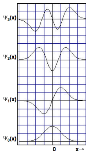
Figure 3: Harmonic oscillator eigenfunctions for n=0, 1, 2, 3 .
