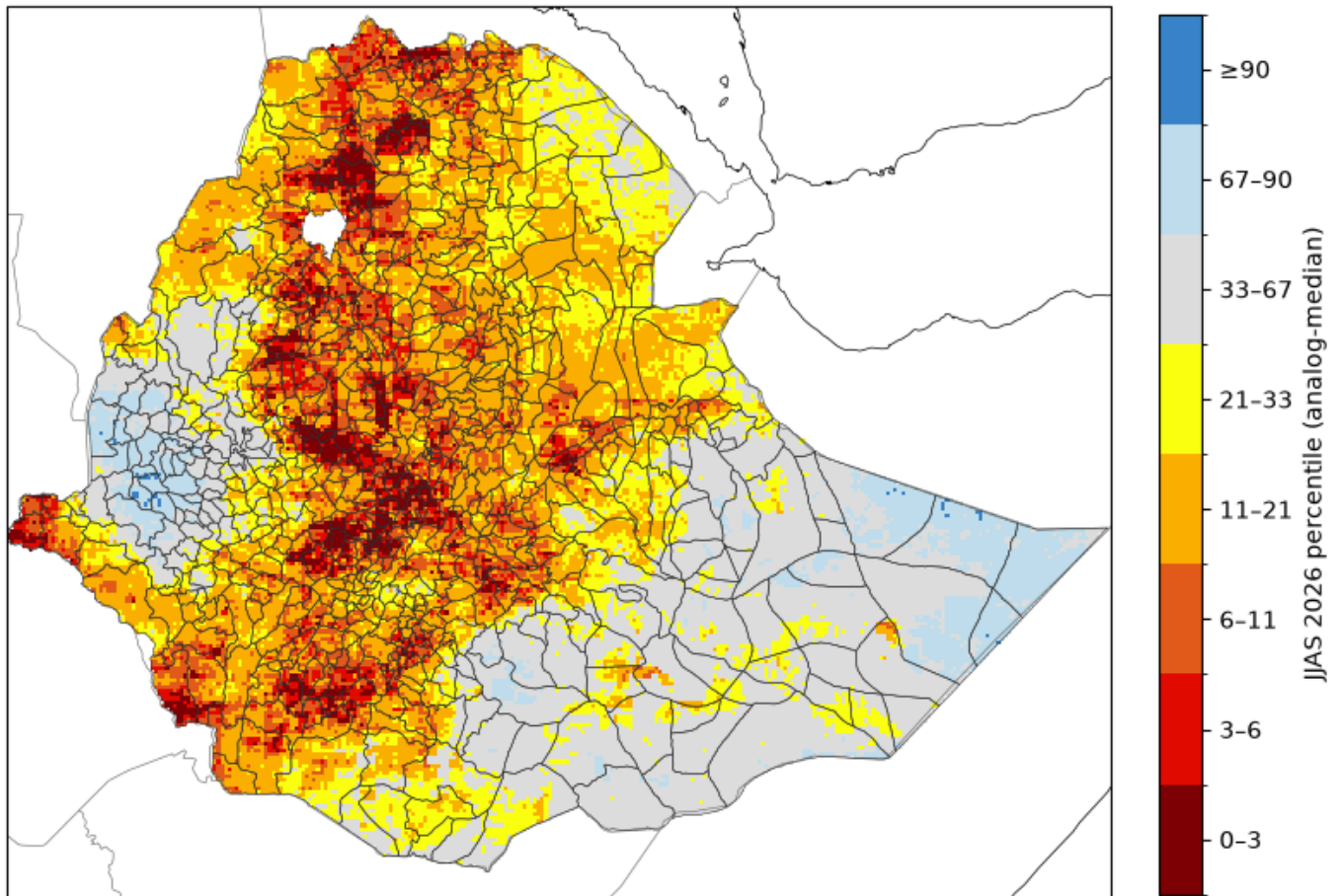
Ethiopia Kiremt 2026 end-of-season outlook (obs + analogs, analog-median)
