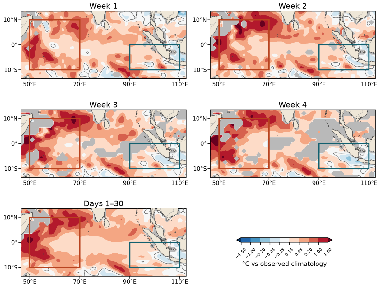
Figure 2: Corrected SST anomaly at every horizon ( ^{\circ}\text{C} vs the 2006–2025 observed average). Boxes: western (orange) and eastern (teal); land in tan. Grey ocean is where leave-one-year-out correlation falls below 0.4 and the forecast should not be relied on; that area expands with lead across the basin, and the eastern box is consistently the more affected. Each cell is corrected by its own regression, observations averaged from 0.25^{\circ} to the model's 1.5^{\circ} grid. Fields are cubic-refined for contouring — presentational only, and the zero contour in particular is placed by the interpolation rather than measured.
