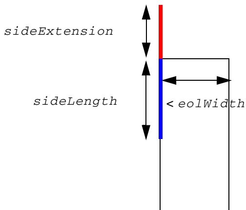
Figure 6-118 Illustration of SIDELENGTH and SIDEEXTENSION
