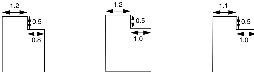
Figure 6-109 MinStep Rule with MINADJACENTLENGTH
