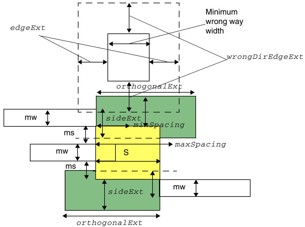
Figure 6-165 Illustration of Spacing Rule with EXCEPTWRONGDIRWIRE in CONVEXCORNERS
