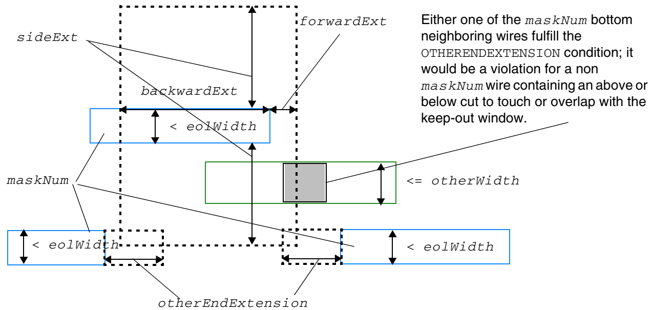
Figure 6-67 Illustrations of EOL Via Keep-out Rule
