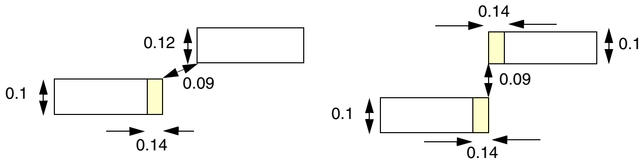
Figure 6-47 EOL Extension Spacing Rule Example
