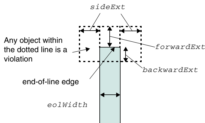
Figure 6-48 Definition of EOL Keep-Out Rule
