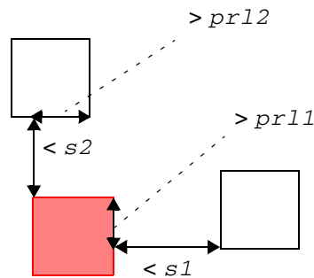
Figure 2-164 Illustration of the Via Group Rule with LGROUP
