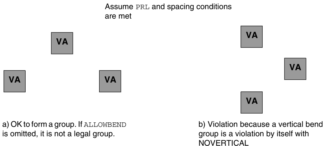
Figure 2-163 Illustration of the Via Group Rule with ALLOWBEND
