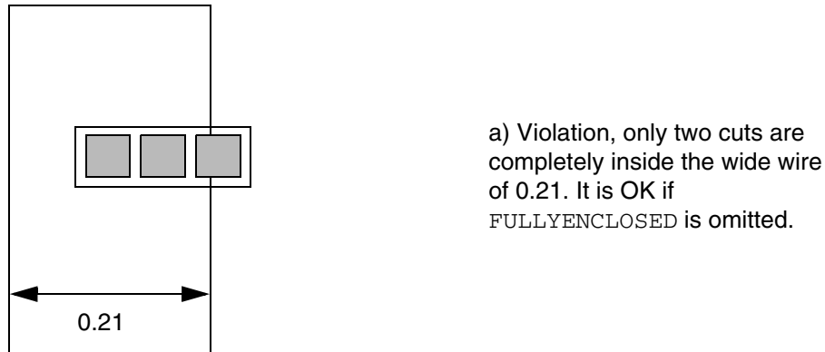
Figure 6-99 Illustration of Minimum Cut Rule with DIFFCUTCLASS and EXCEPTOTHERWIDTH
