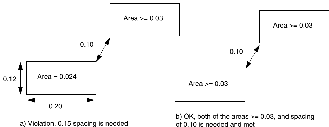
Figure 6-169 Illustration of Spacing Area Rule
