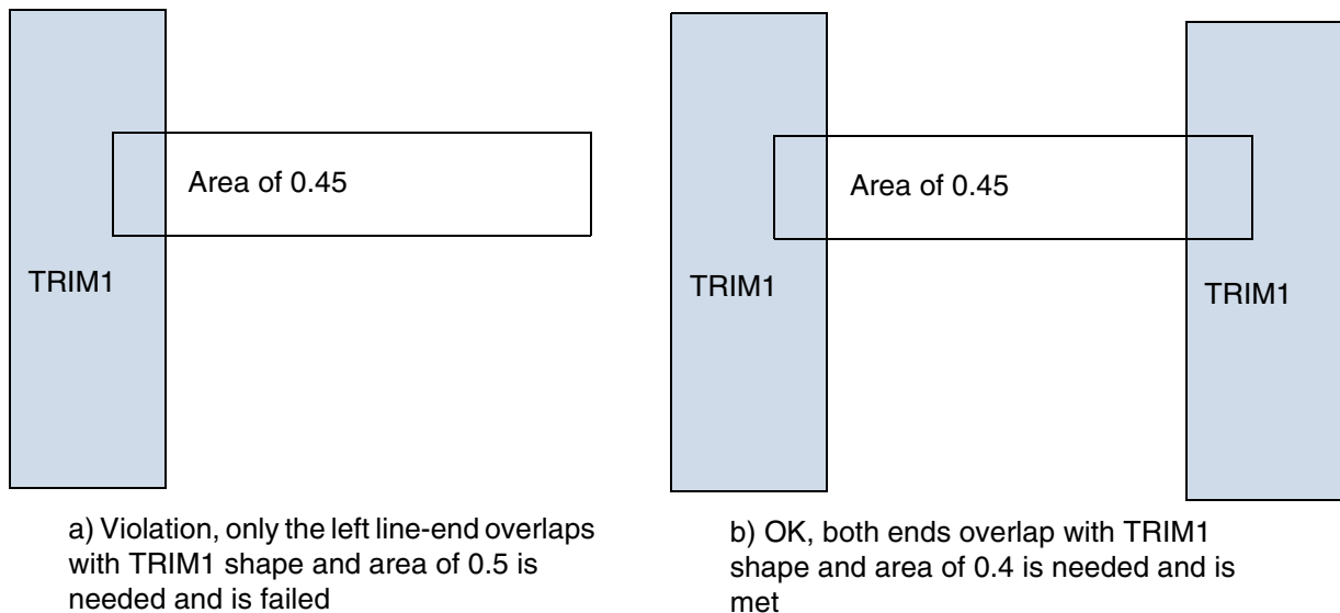
Figure 6-21 Area Rule for Trim Layer with Overlap
