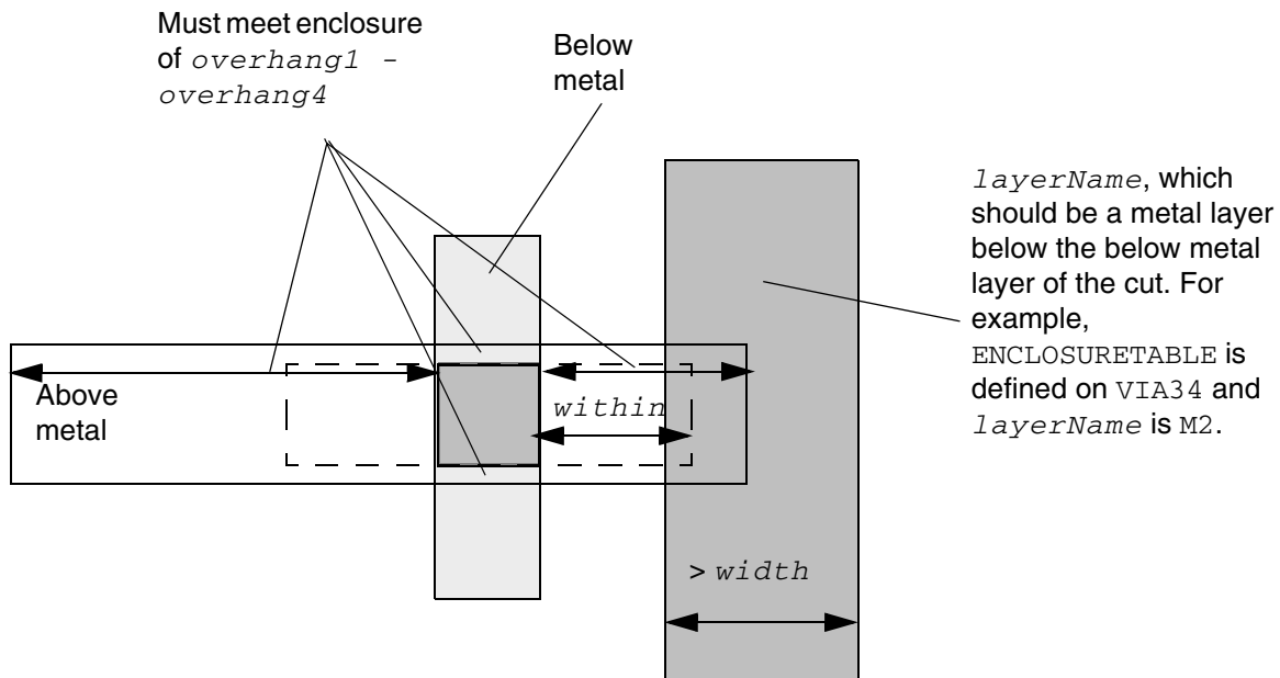
Figure 2-60 Illustration of Enclosure Table Rule with ABOVE OTHERWITHINWIDTH
