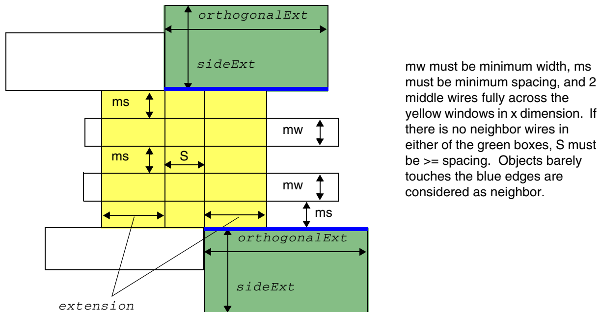
Figure 6-160 Illustration of Spacing Rule with CONVEXCORNERS
