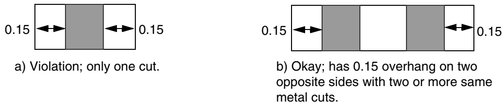
Figure 2-34 Illustration of the Enclosure Rule With CutClass
