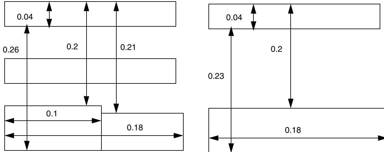
Figure 6-71 Illustration of FORBIDDENSPACING with WIDTH and PRL
