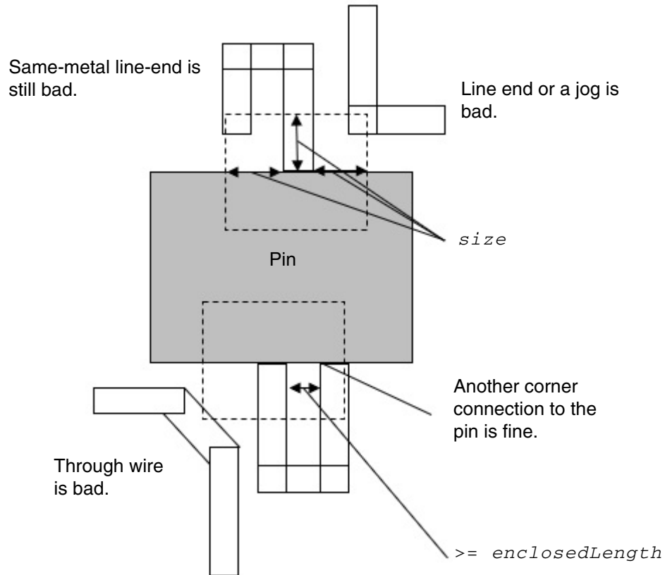
Figure 6-123 Example of a Pin Connect Blockage Rule
