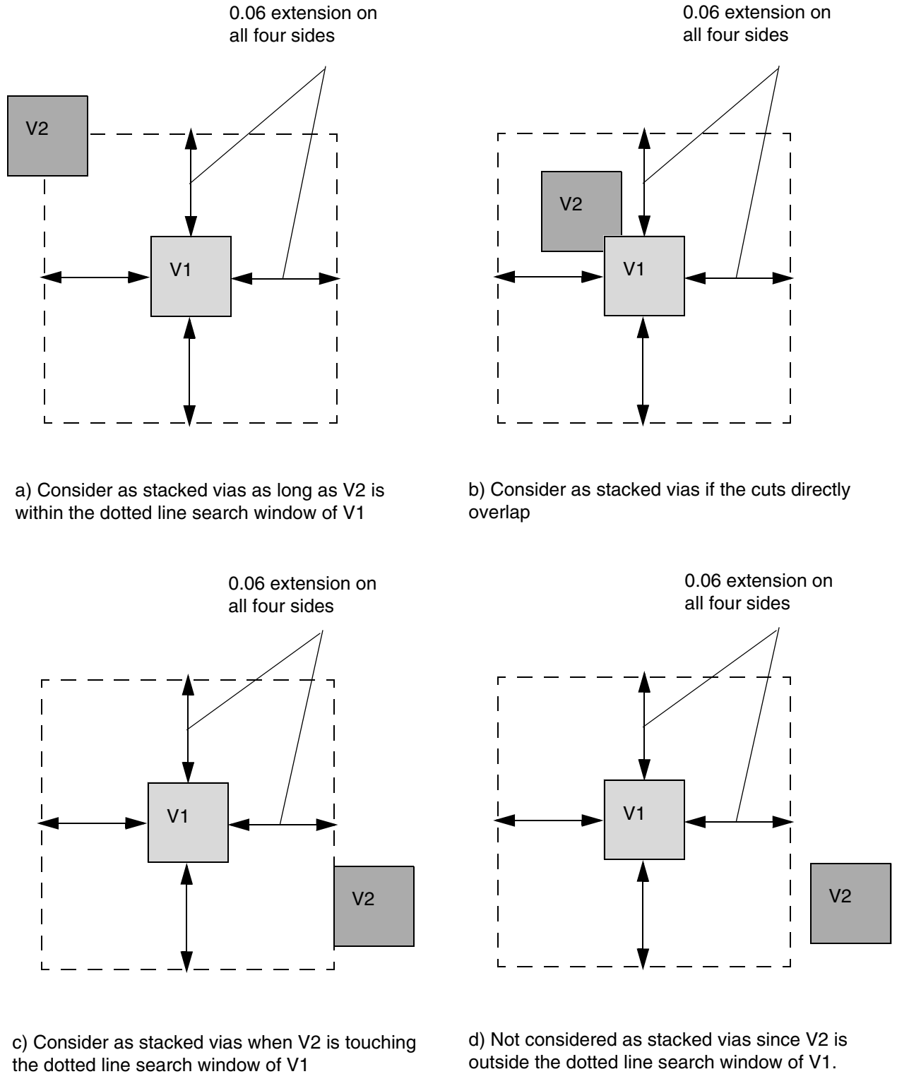
Figure 1-15 Illustration of Max Via Stack Rule with WITHIN LOWCUTSIZE
