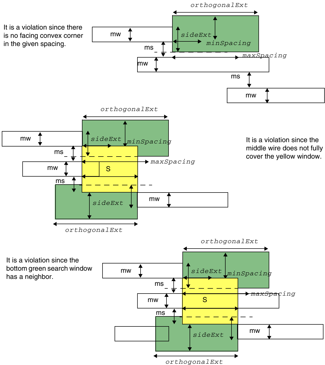
Figure 6-164 Illustrations of Spacing Rule with REVERSE in CONVEXCORNERS
