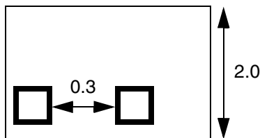
Figure 6-2 Minimum Cut Within Rule
