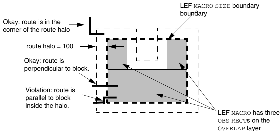
Figure 7-2 Route Halo
