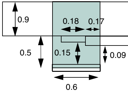
Figure 6-183 Illustration of Spacing Table with JOGTOJOGSPACING
