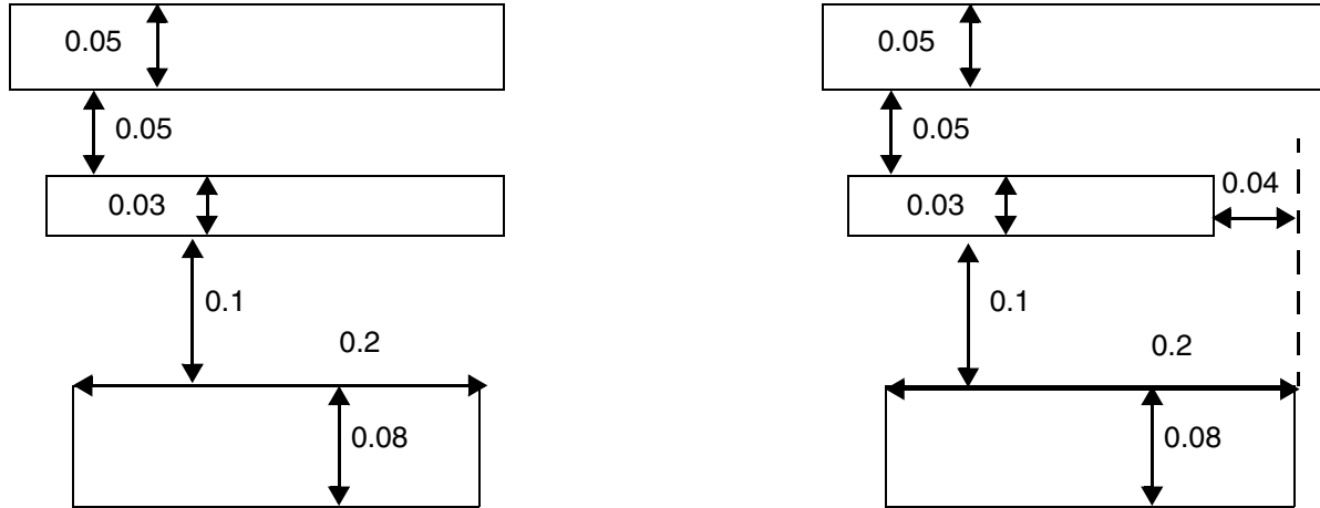
Figure 6-199 Illustration of TWOWIRESFORBIDDENSPACING with IGNOREMIDDLE
