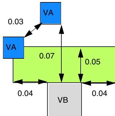
Figure 2-26 Illustration of the Directional Spacing Rule
