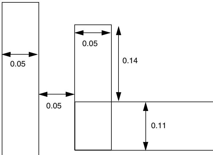
Figure 6-196 Illustration of PARALLELRUNLENGTH with WRONGDIRECTION
