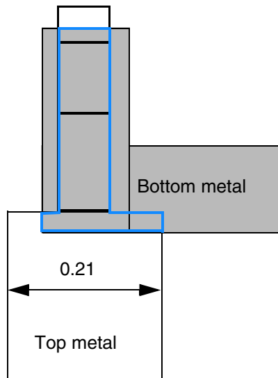
Figure 6-97 Illustration of Minimum Cut Rule with SAMEMETALOVERLAP
