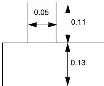
Figure 6-125 Illustration of Protrusion Width Rule
