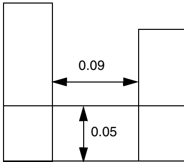
Figure 6-178 Illustration of Spacing Rule with EXCEPTWITHIN and NOTCHWIDTH
