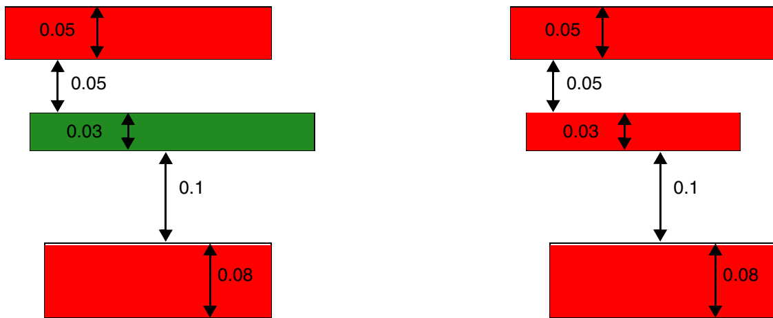
Figure 6-197 Illustration of TWOWIRESFORBIDDENSPACING
