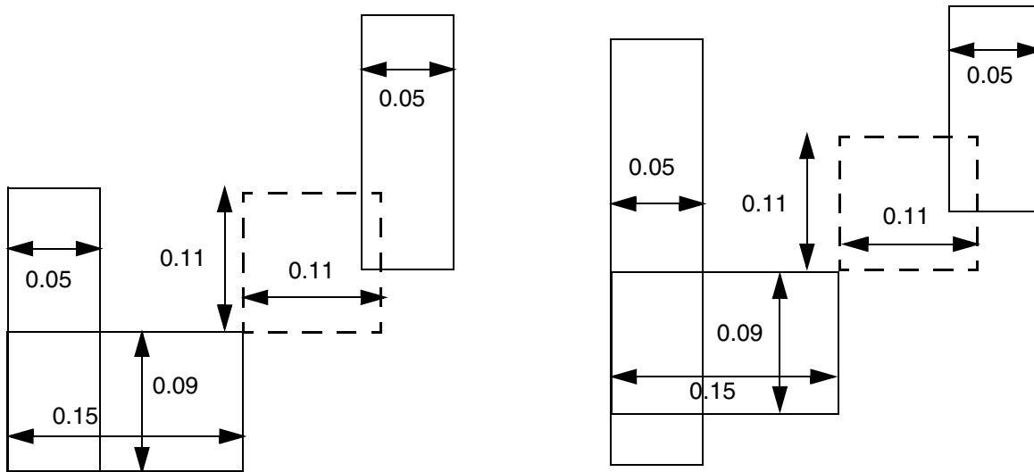
Figure 6-34 Illustration of Corner Spacing Rule
