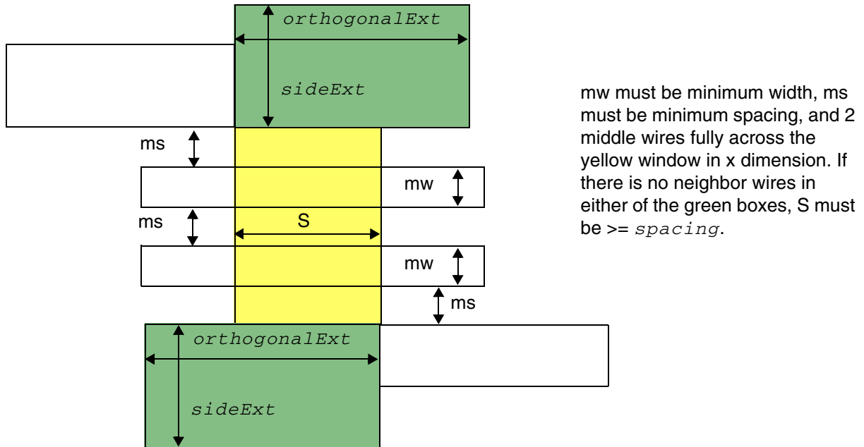
Figure 6-159 Illustration of Spacing Rule with CONVEXCORNERS
