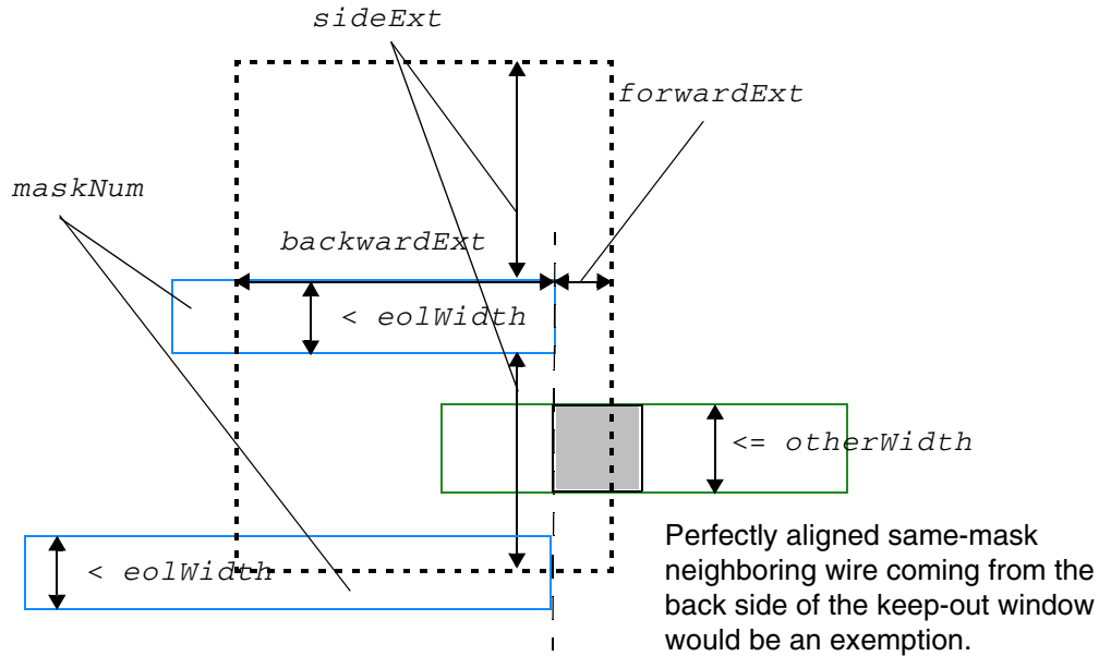
Figure 6-68 Illustration of EOL Via Keep-out Rule with EXCEPTBACKSIDEALIGNED
