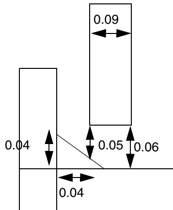
Figure 6-157 EOL Spacing Rule with EXCEPTEXACTWIDTH
