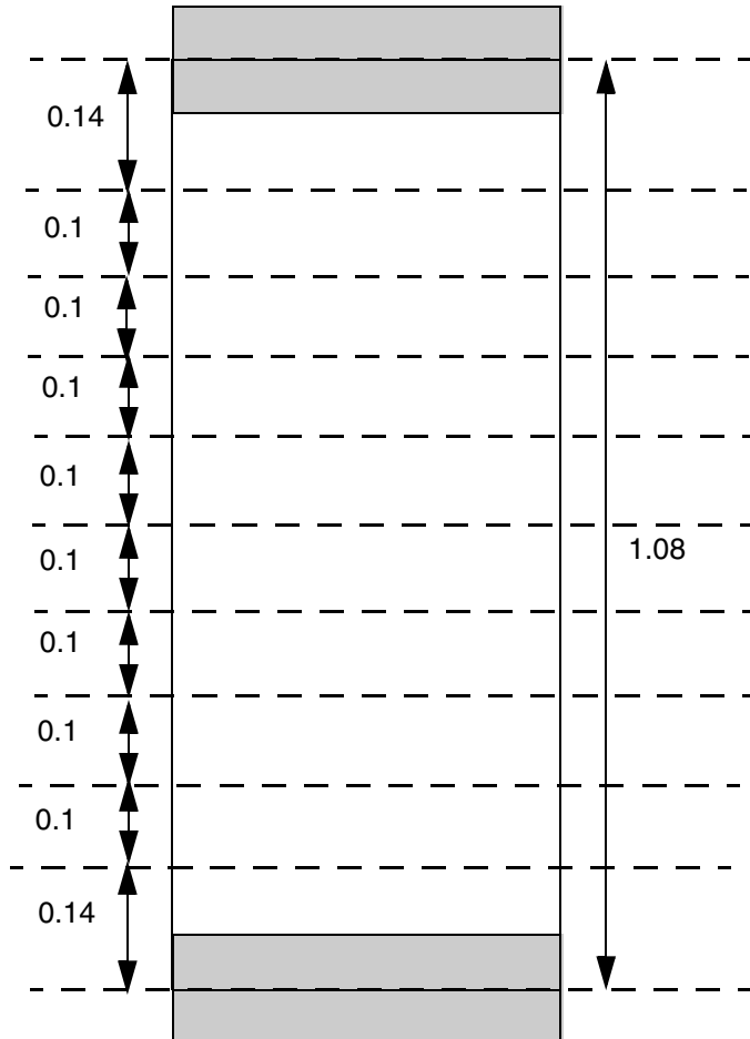
Figure 6-124 Example of Pitch Rule
