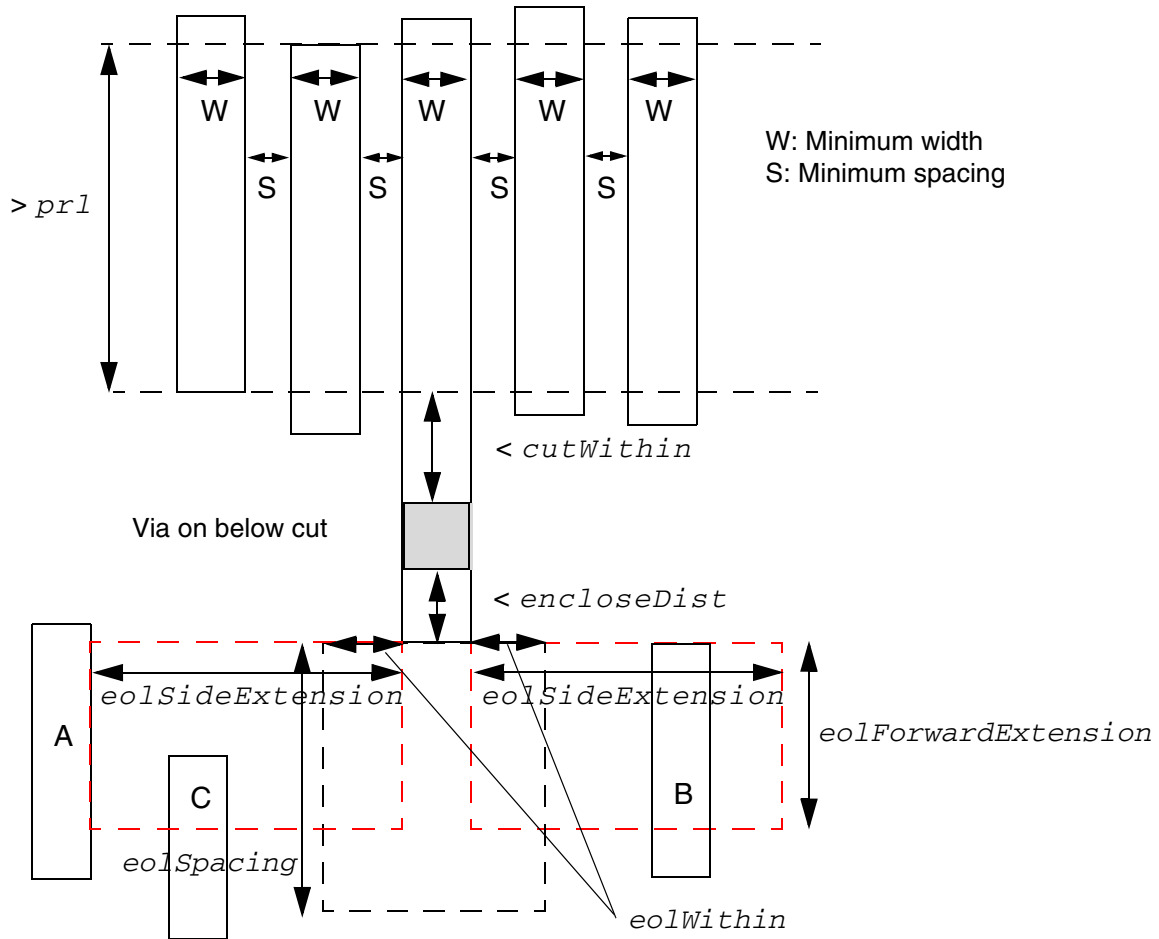
Figure 6-69 Illustration of FIVEWIRESEOLSPACING
