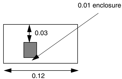
d) OK, EOL edges are exempted from the rule
