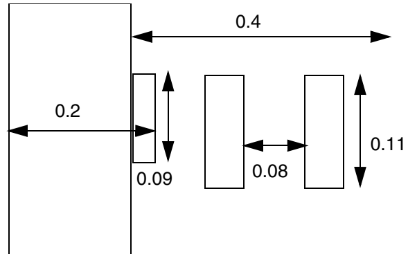
Figure 6-72 Illustration of FORBIDDENSPACING with WIDTH and WITHIN
