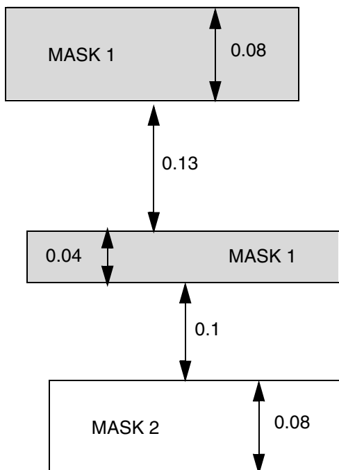
Figure 6-81 Illustration of FORBIDDENSPACING with WIDTHRANGE
