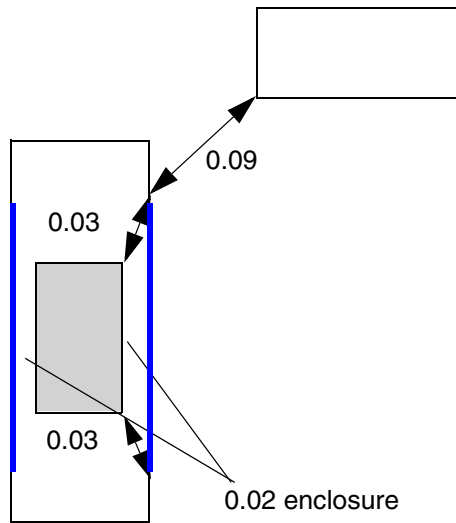
Figure 6-39 Illustration of Enclosure Spacing Rule
