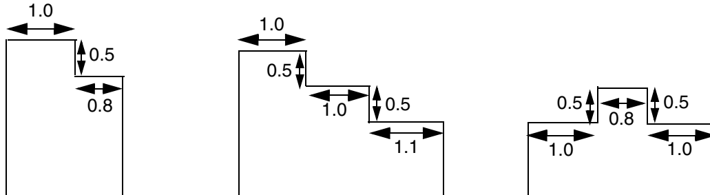
Figure 6-108 MinStep Rule with Adjacent Edge
