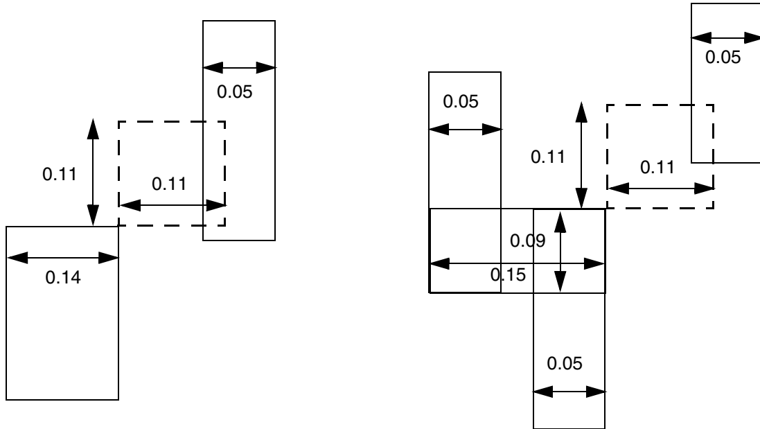
Figure 6-33 Illustration of Corner Spacing Rule
