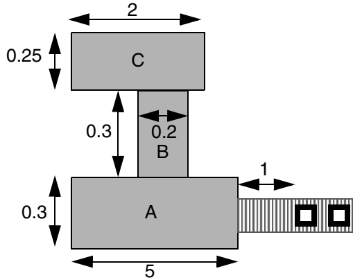
Figure 6-96 Minimum Cut Rule Example
