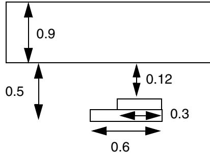
Figure 6-182 Illustration of Spacing Table with JOGTOJOGSPACING
