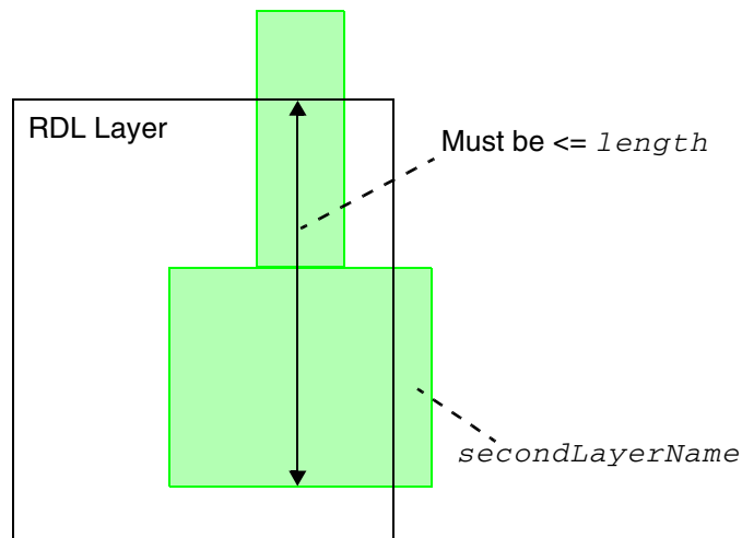
Figure 6-93 Illustration of Maximum Overlap Length Rule
