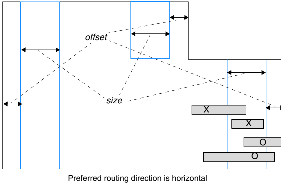
Figure 6-24 Illustration of the Boundary EOL Blockage Rule
