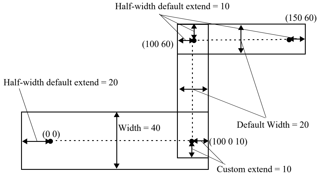
Figure 7-6 Routing Points - Usage of Width
