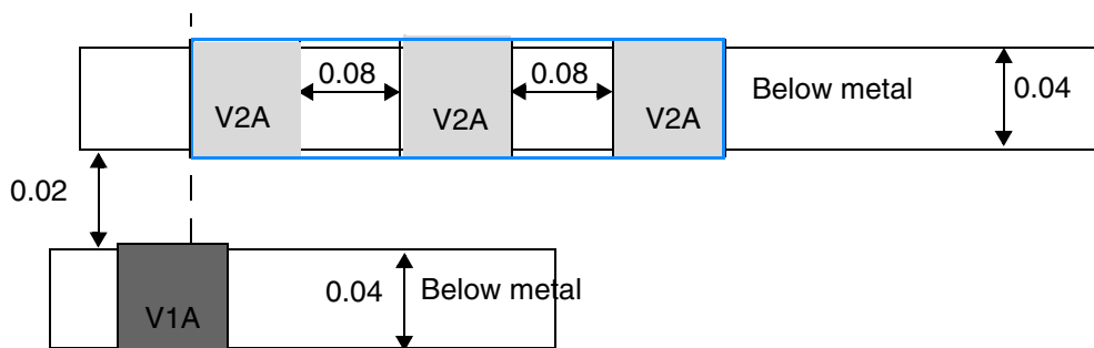
Figure 2-157 Illustration of the Same-Metal Aligned Cuts Rule with CUTWITHIN
