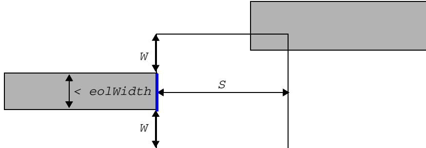
Figure 6-66 Illustration of EOL Track Rule with WITHIN in EXCEPTEOLSPACING
