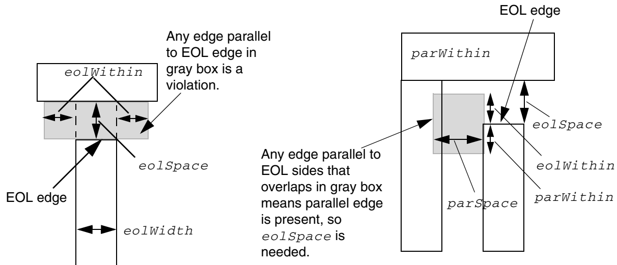
Figure 6-149 EOL Spacing Rule Illustrations
