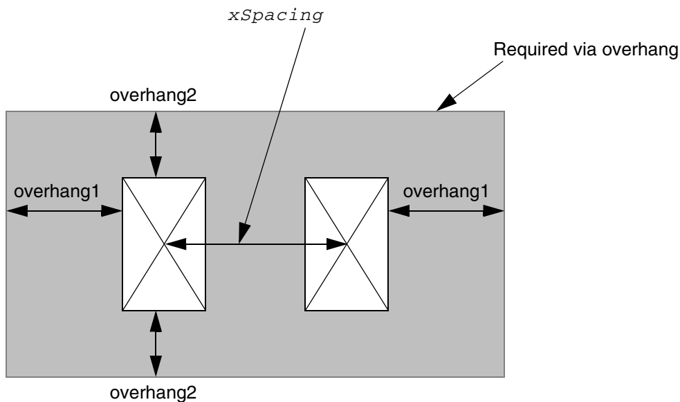
Figure 1-68 Overhang
