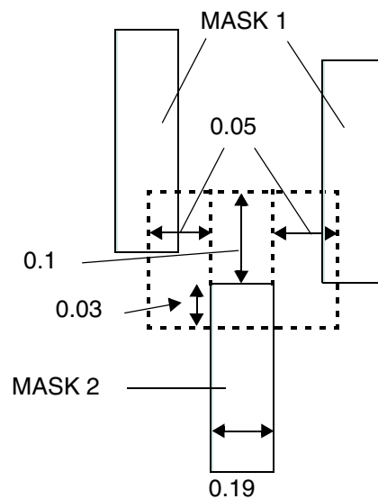
Figure 6-56 Illustration of EOL Keep-Out Rule with Mask and Two Sides
