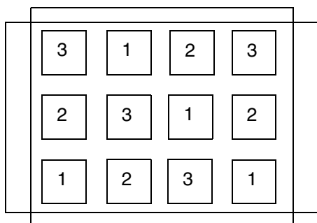
Figure 7-8 Multi-Mask Patterns with Special Wiring
