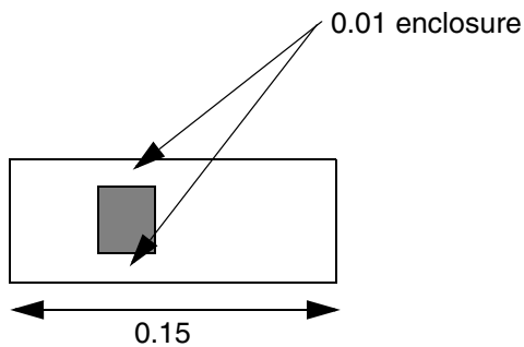
c) OK, 0.01 enclosure on 2 entire opposite edges
