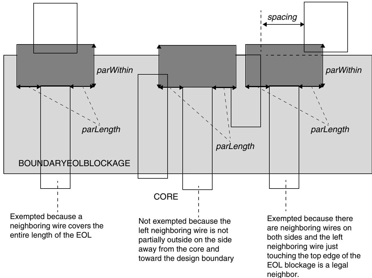
Figure 6-25 Illustration of the Boundary EOL Blockage Rule with PARALLEL, WITHIN, and SPACING
