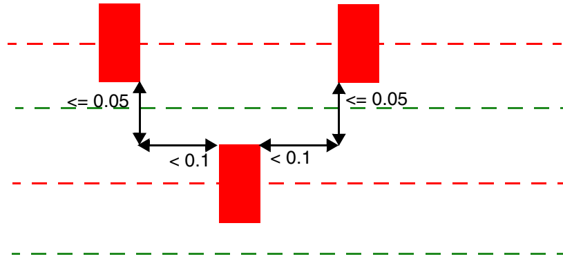
Figure 4-5 Example of Adjacent Trim Rule with WITHIN
