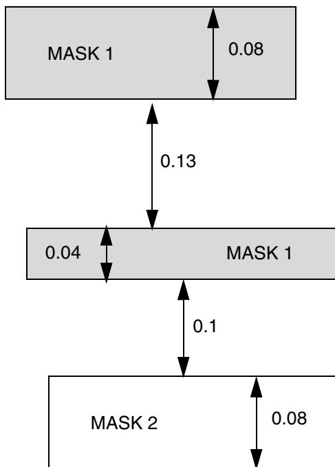
Figure 6-82 Illustration of FORBIDDENSPACING with OTHERSAMEMASK
