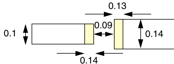
Figure 6-44 EOL Extension Spacing Rule Example
