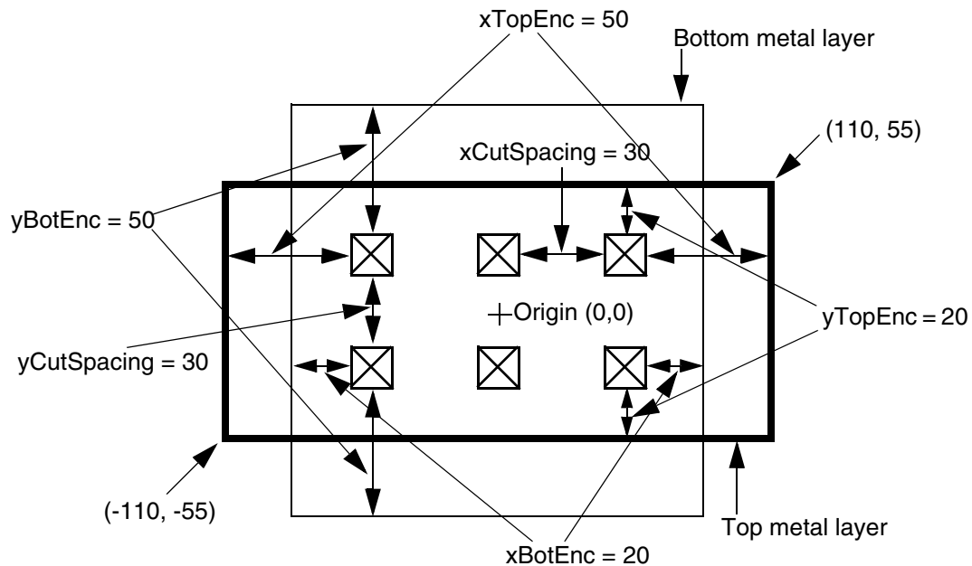
Figure 1-62 Via Rule
