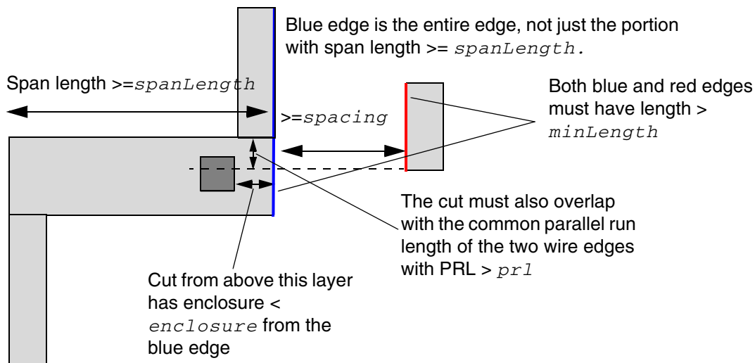
Figure 6-136 Illustration of SPANLENGTHENCLOSURESPACING
