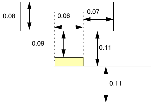
Figure 6-195 Illustration of Spacing Table Rule with EXCEPTWITHIN
