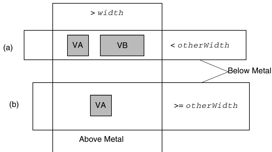
Figure 6-99 Illustration of Minimum Cut Rule with DIFFCUTCLASS and EXCEPTOTHERWIDTH
