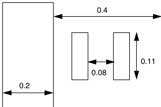
Figure 6-72 Illustration of FORBIDDENSPACING with WIDTH and WITHIN
