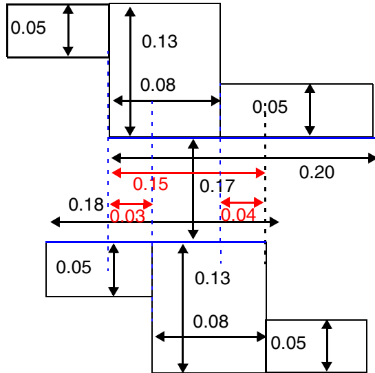
Figure 6-202 Illustration of TWOWIRESFORBIDDENSPACING with OTHERSPANLENGTH
