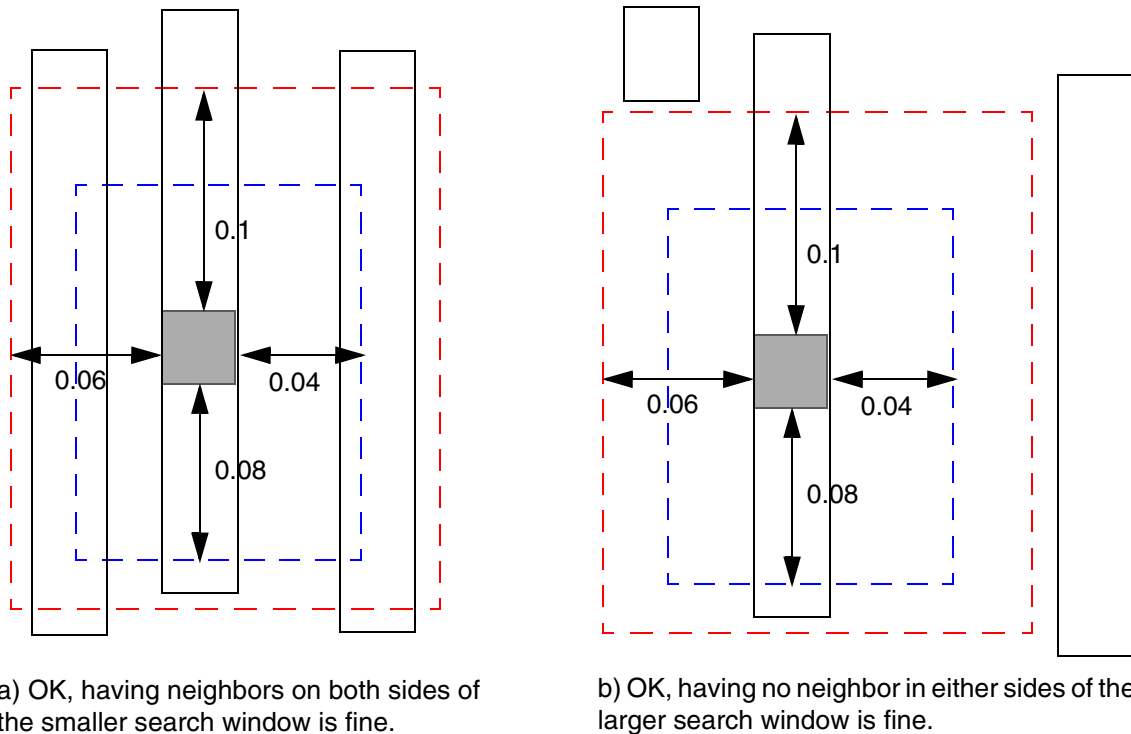
Figure 2-41 Illustration of the Enclosure Rule With PARALLEL and WITHIN
