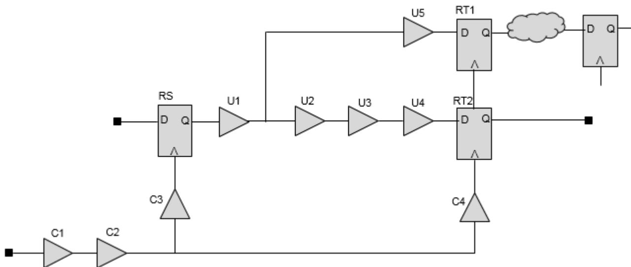
Figure 4-69 Launch cell and net stage counts
