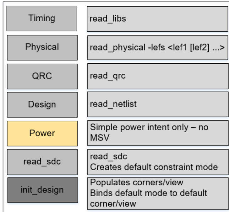
Figure 4-2 Base Delay Analysis Initialization Flow - Non-MMMC Mode
