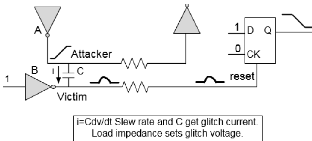
Figure 4-43 Glitch due to SI resulting in functional failure
