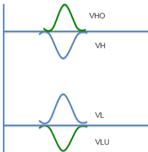
Figure 4-54 VL, VH, VLU, and VHO glitch waveforms
