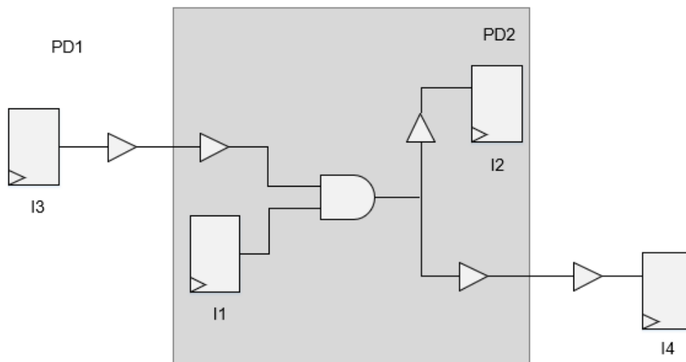
Figure 4-83 Non-IPD Path Analysis - Illustration
