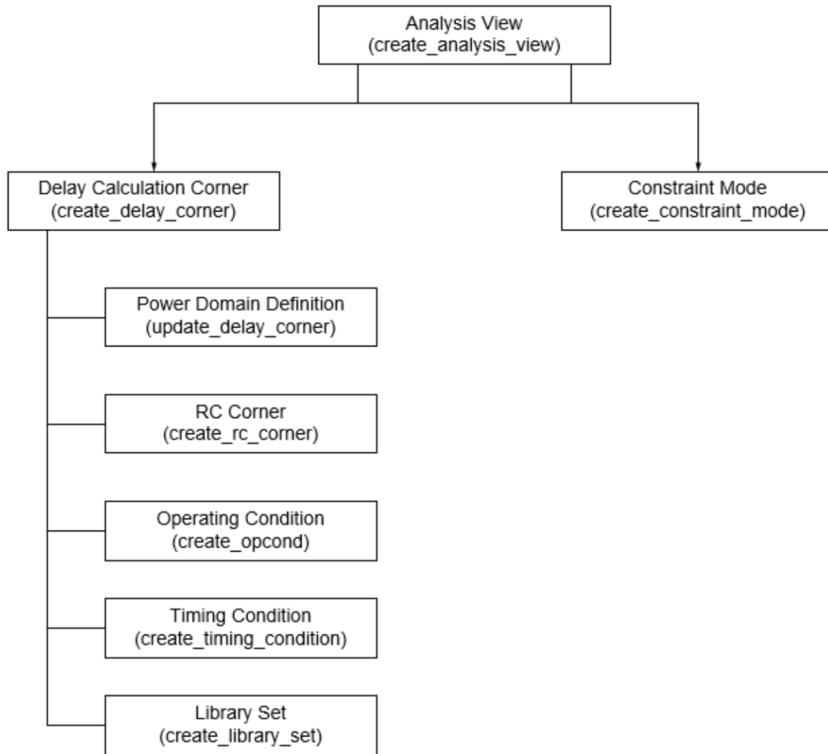
Figure 5-1 Hierarchical Analysis View Configuration
