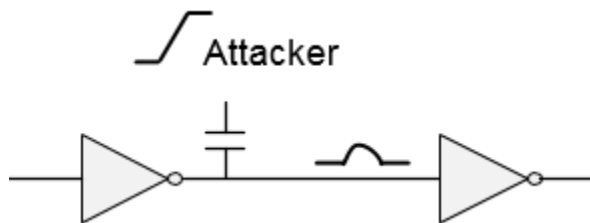
Figure 4-53 VLU Glitch
