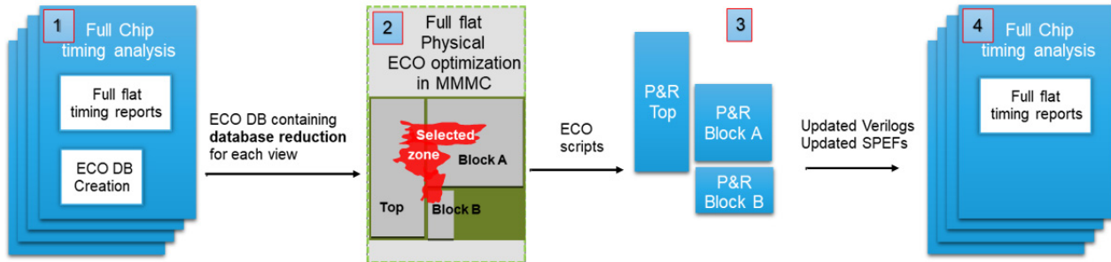
Figure 8-8 Steps for Completing STA
