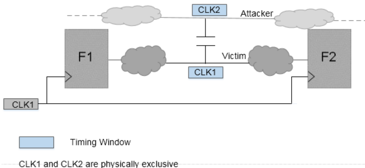
Figure 4-32 Attackers receiving TW with respect to Physically exclusive clock
