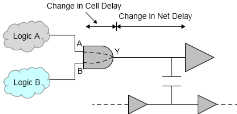
Figure 4-42 SI Impact on Delay Computed on Timing Arc
