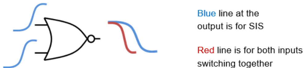
Figure 4-105 NOR-2 gate has parallel n-stacks both discharge output when turned on
