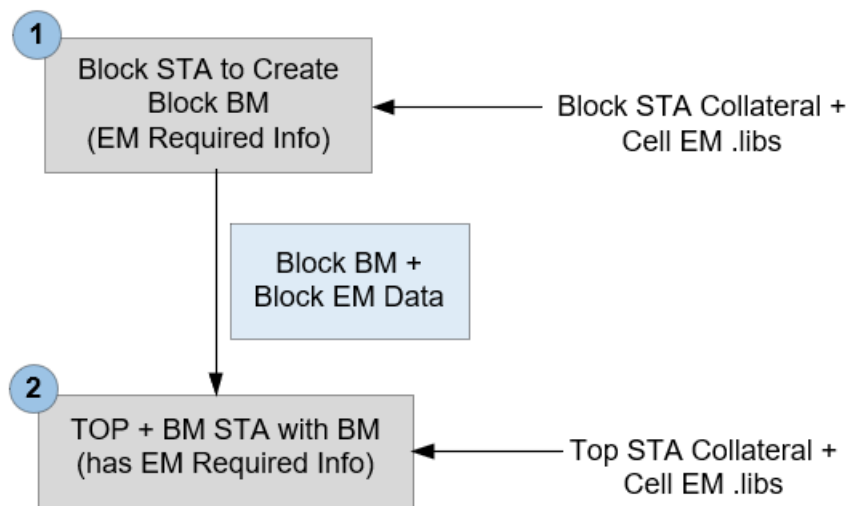
Figure 4-123 Cell EM Boundary Model-Based Flow
