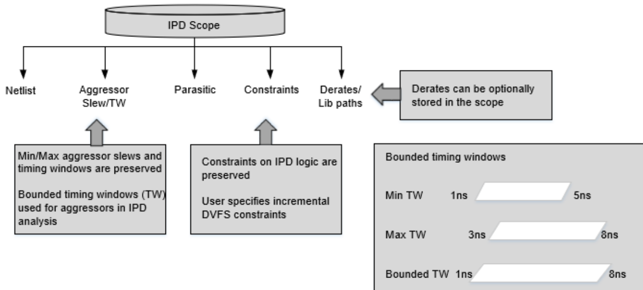
Figure 4-80 Scope Based IPD Analysis
