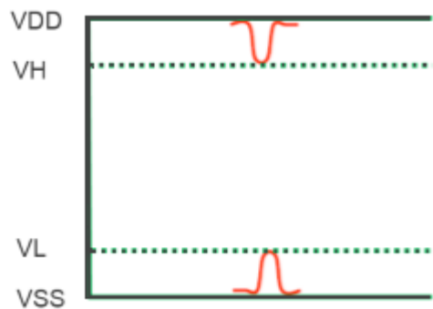
Figure 4-44 VL and VH Glitch type
