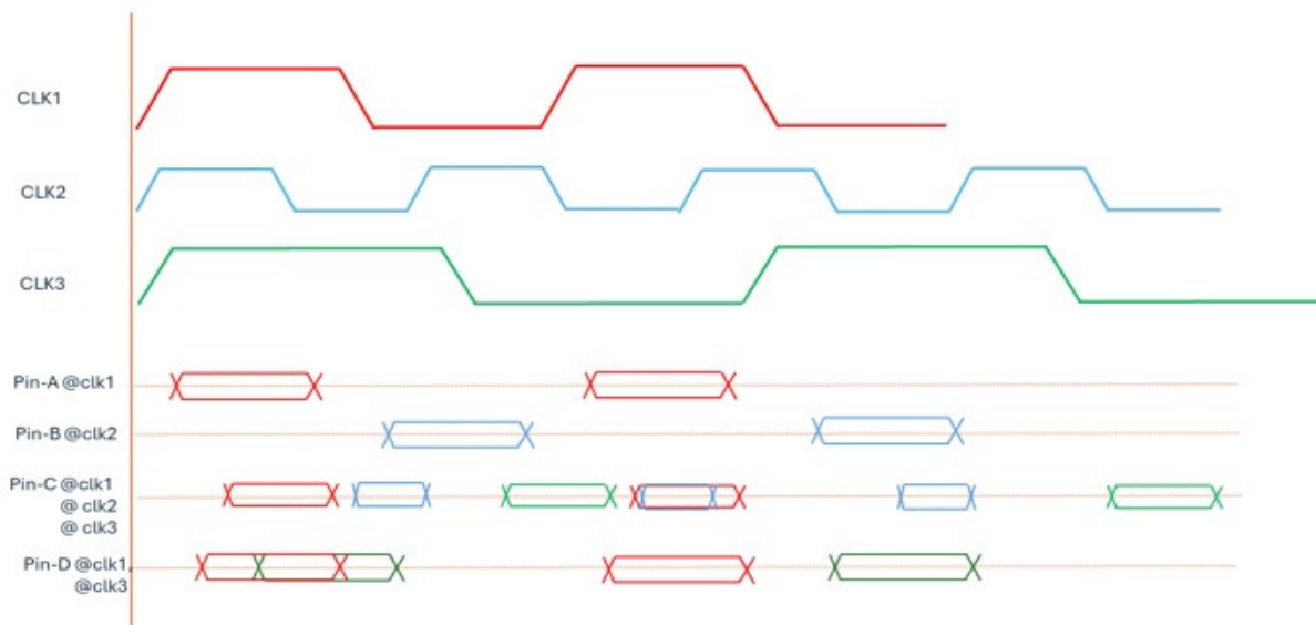
Figure 4-118 Clock-groups have no impact on AMIS-derate
