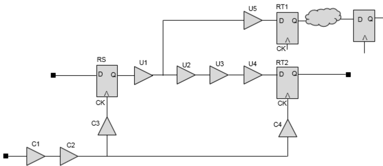
Figure 4-68 Timing Paths
