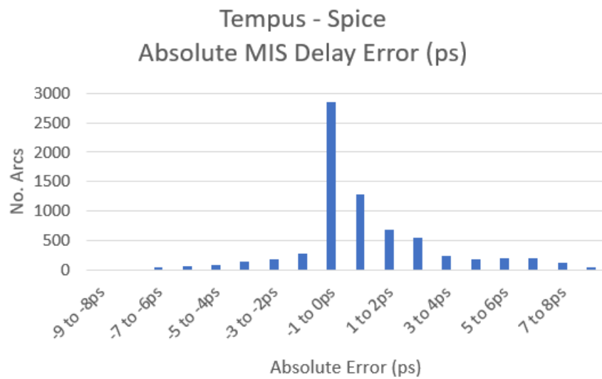
Figure 4-114 Negative error: Tempus more pessimistic than Spice
