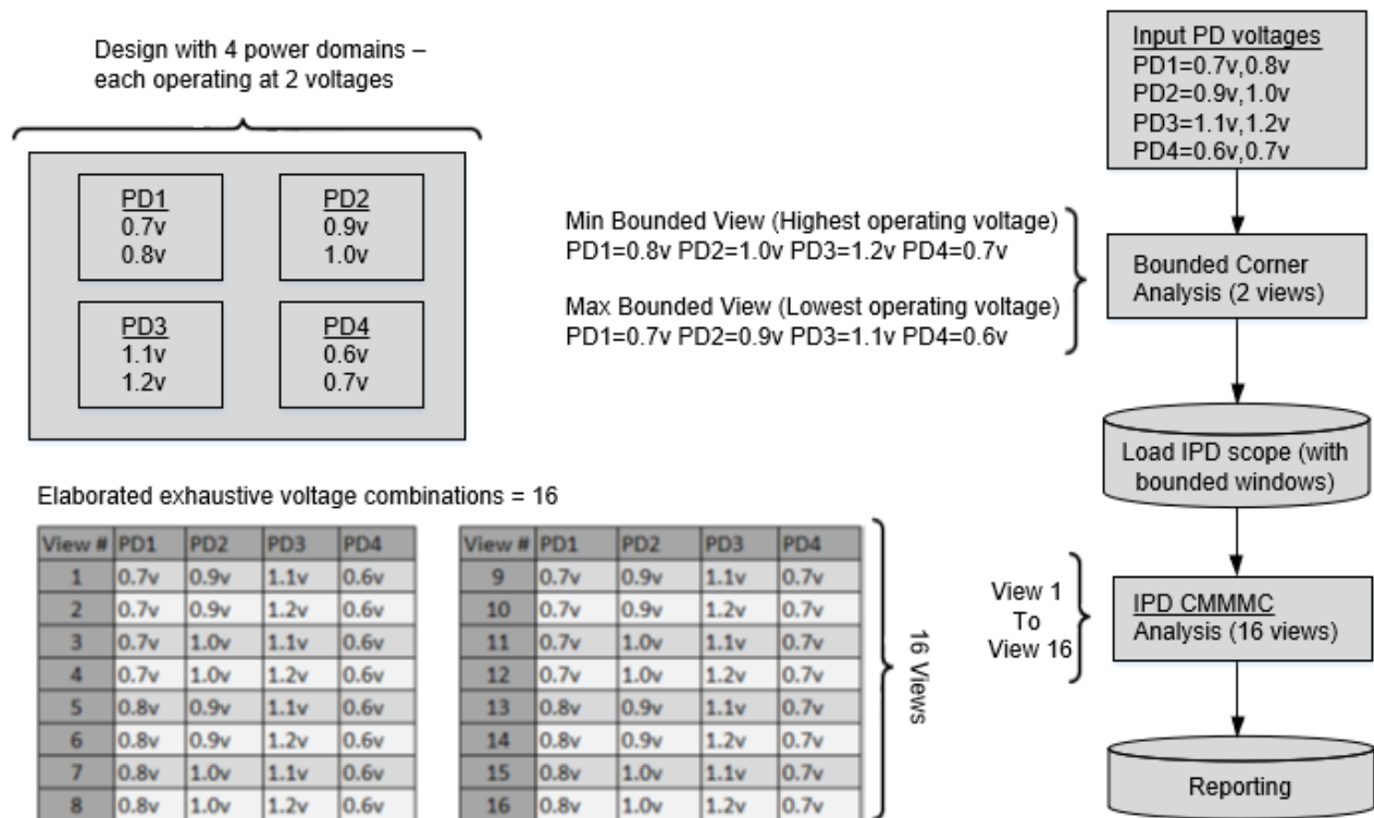
Figure 4-82 Scope Based IPD Analysis - Illustration
