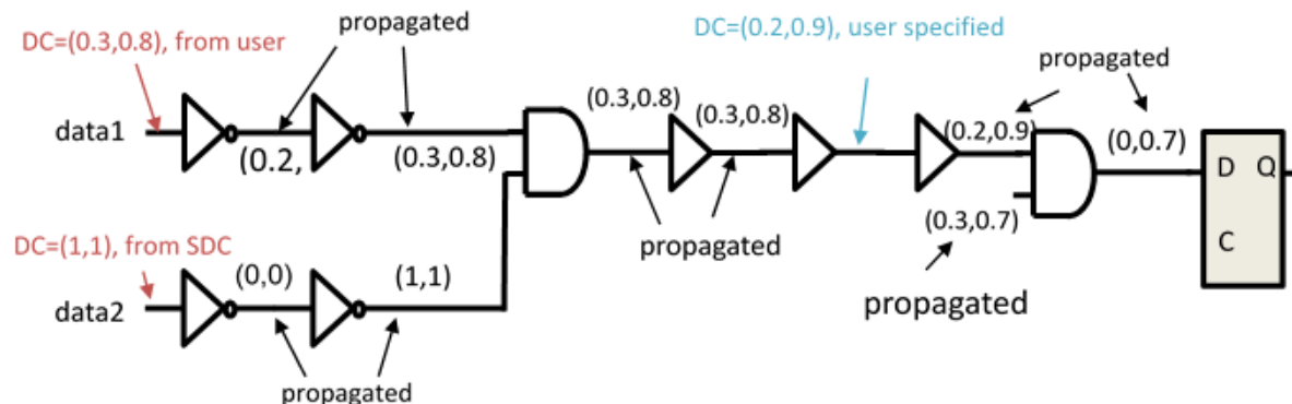
Figure 4-99 Duty cycle propagation for data path (Worst-case)
