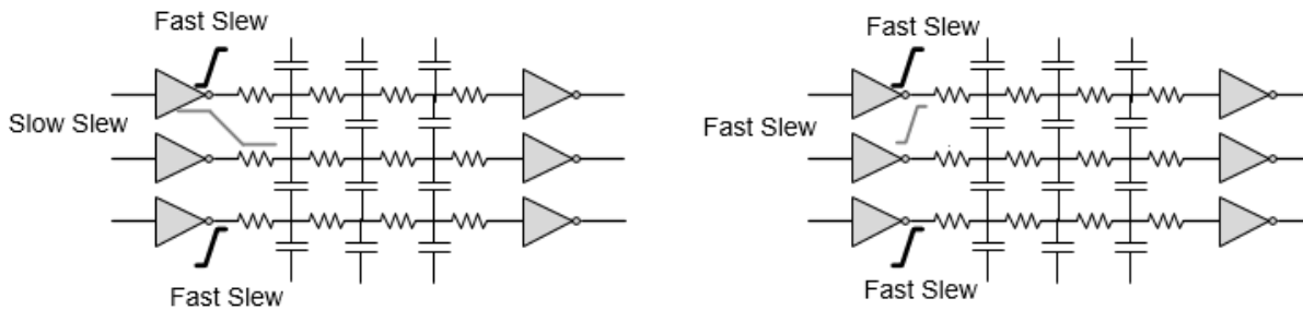
Figure 4-37 Determine slew for max delay and min delay
