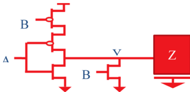
Figure 4-106 NOR gate showing speed-up with two inputs rising.
