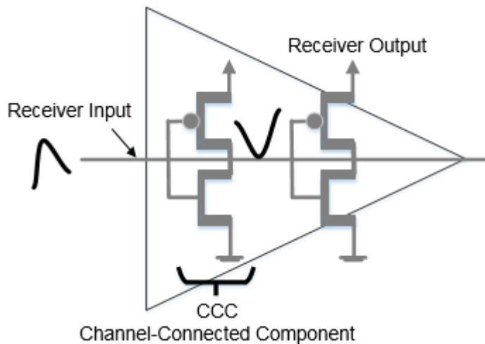
Figure 4-46 Glitch representation at input and output of receiver
