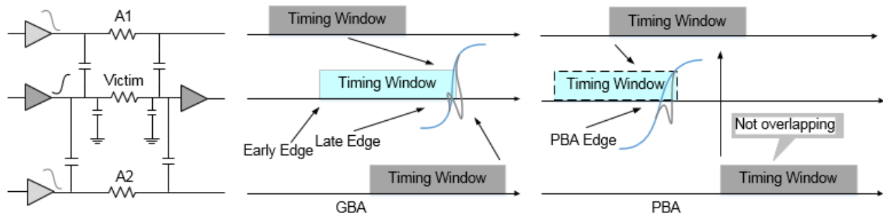
Figure 4-22 Path Overlap Alignment Mode
