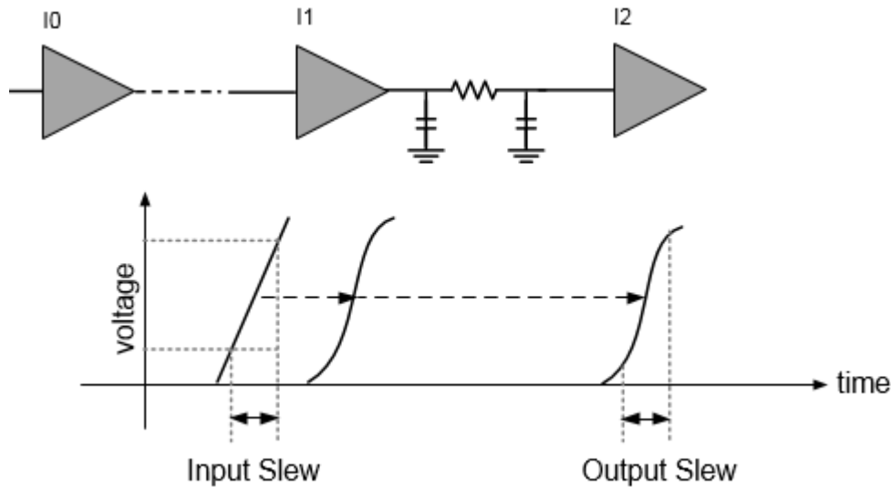
Figure 4-4 Traditional Delay Calculation using Delay as function of slew and load
