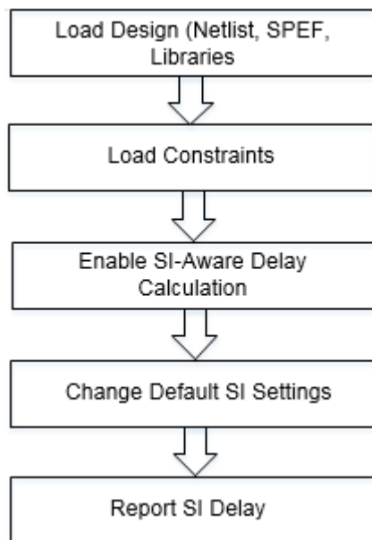
Figure 4-12 Tempus SI Delay Analysis Flow
