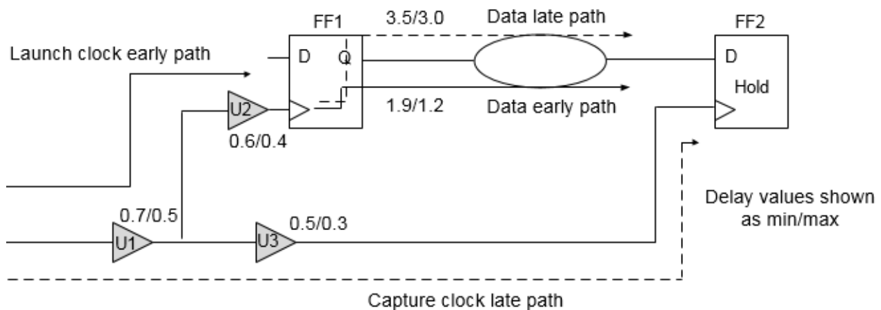
Figure 4-65 Hold Check in OCV Mode
