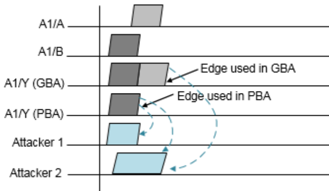
Figure 4-27 Timing-Aware Edge Mode
