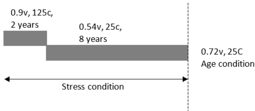
Figure 4-97 Stress Profile
