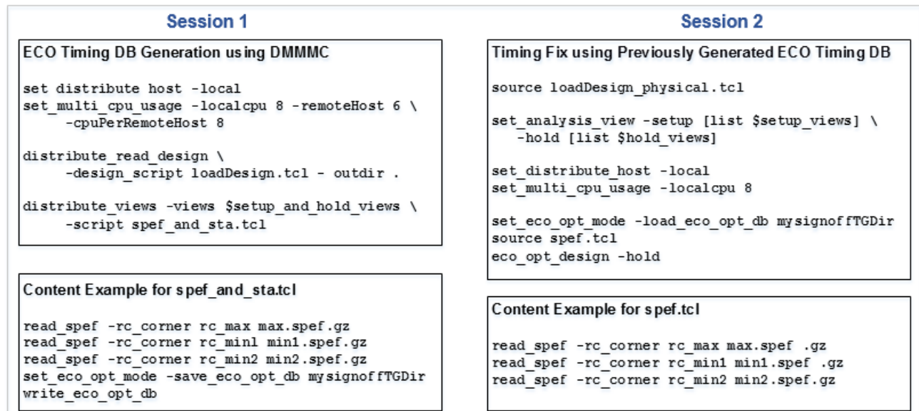
Figure 8-2 ECO Timing Closure in Separate Sessions
