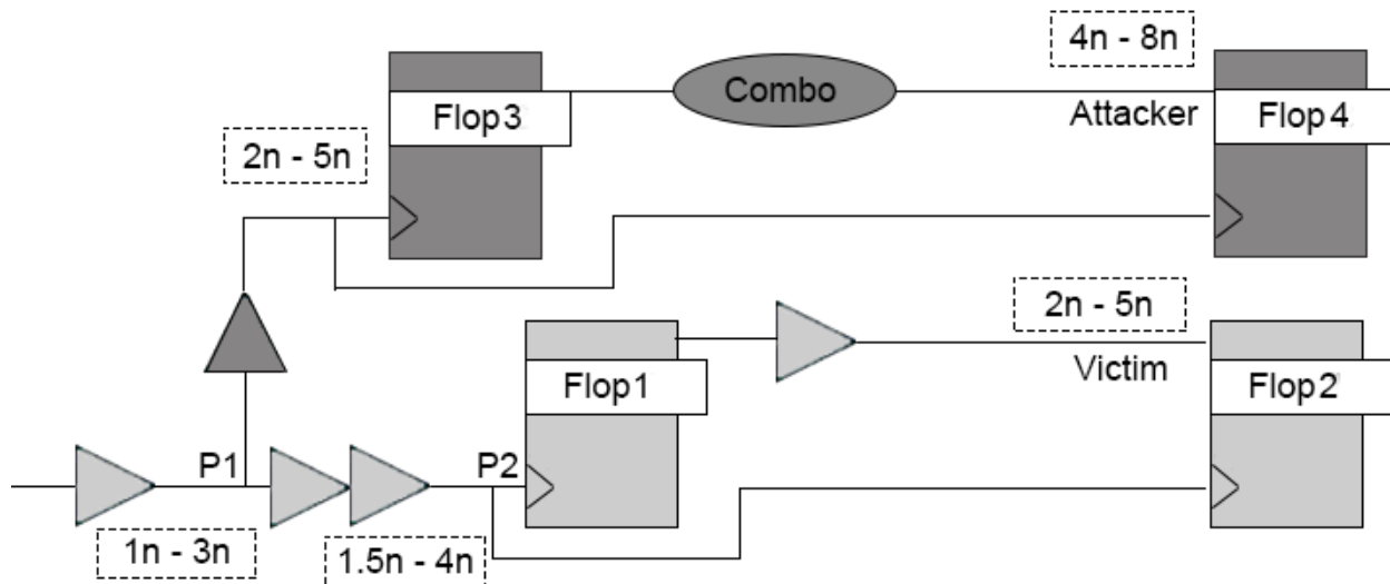
Figure 4-17 Timing Windows on CPPR Mode
