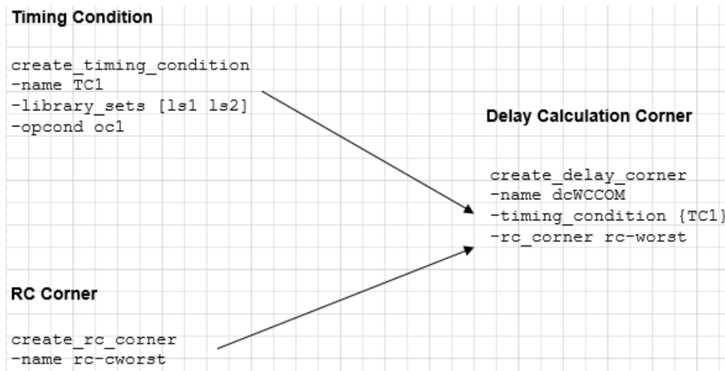
Figure 5-4 Creation of a delay calculation corner
