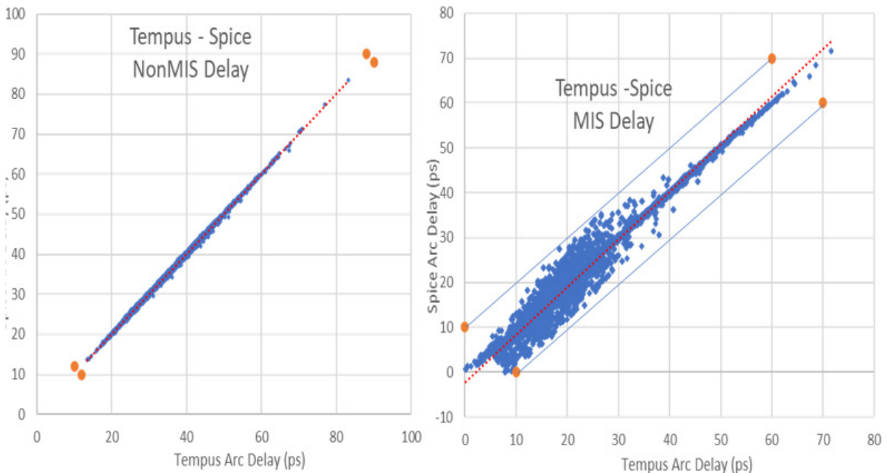
Figure 4-113 Spice accuracy results
