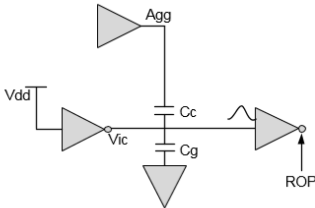
Figure 4-47 ROP (Receiver Output Peak) for single stage cell
