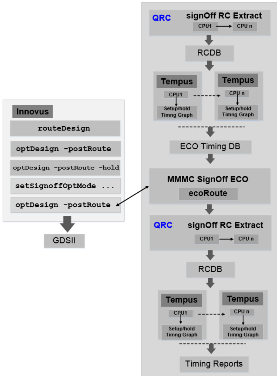
Figure 8-5 Signoff Timing Optimization Flow
