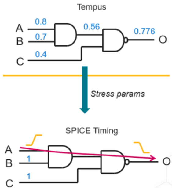
Figure 4-104 Method 2 (Timing-only correlation)
