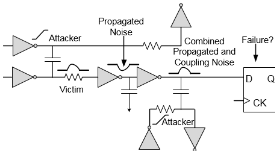
Figure 4-51 Glitch Propagation
