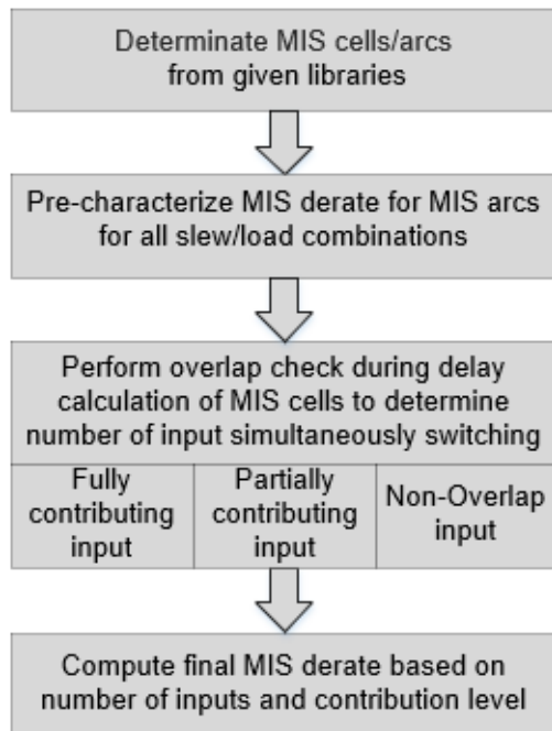
Figure 4-115 AMIS Derate Flow
