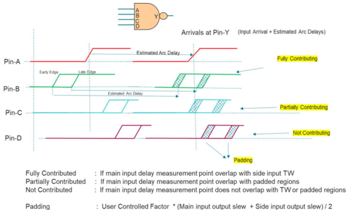
Figure 4-116 Overlap check
