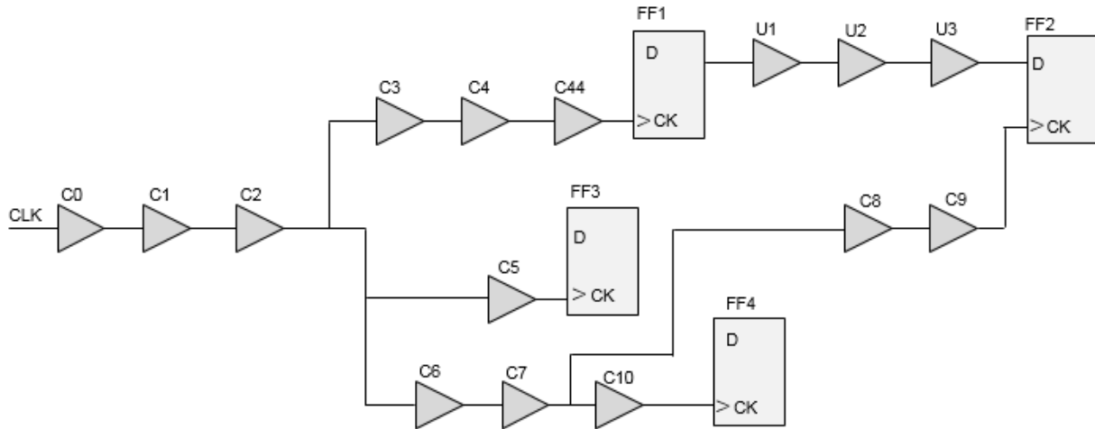
Figure 4-72 AOCV stage count
