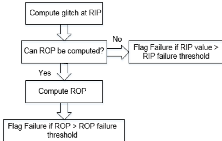
Figure 4-50 Glitch Failure Flow
