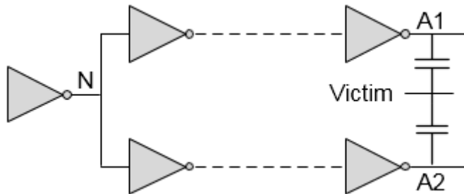
Figure 4-36 Logical Relationship Between Remote Attackers
