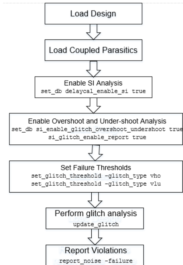
Figure 4-55 Overshoot-Undershoot Analysis Flow
