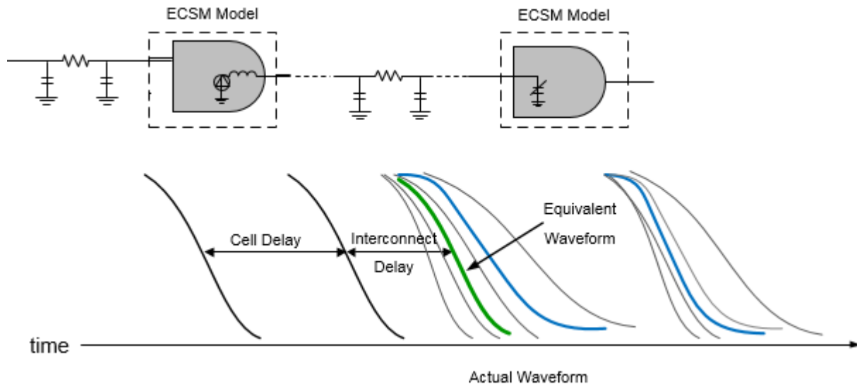
Figure 4-8 Delay Calculation with EWM
