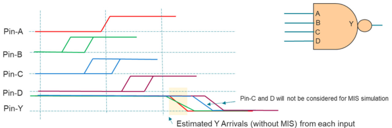
Figure 4-110 Overlap alignment mode
