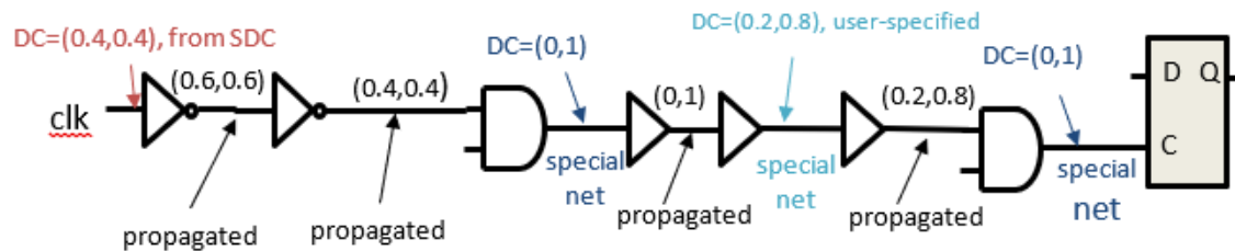
Figure 4-98 Duty cycle propagation through clock network (Worst-case)
