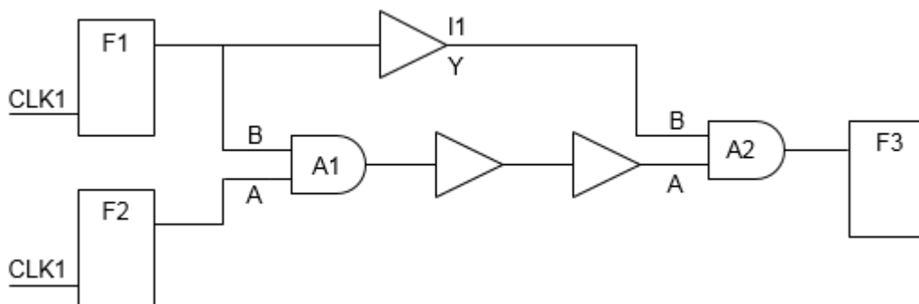
Figure 4-26 Timing-Aware Edge Mode - Example 1
