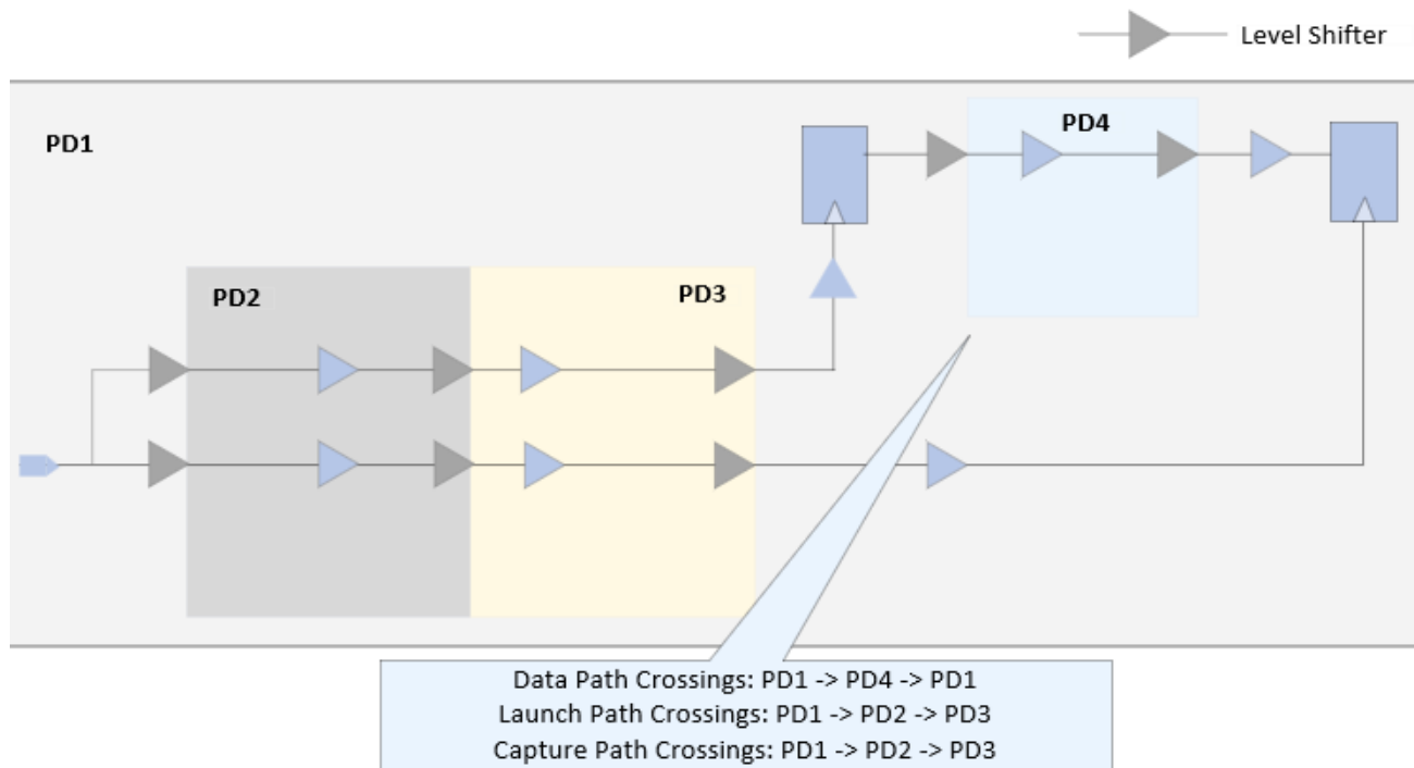
Figure 4-92 Multiple PDs post common point
