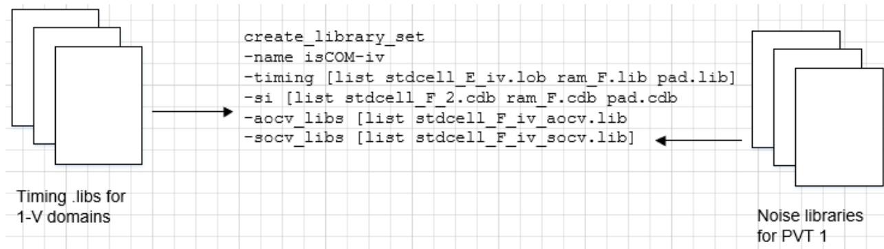
Figure 5-2 Creation of Library Sets
