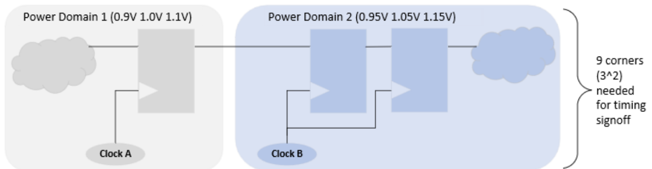
Figure 4-85 IPD Signoff Corners
