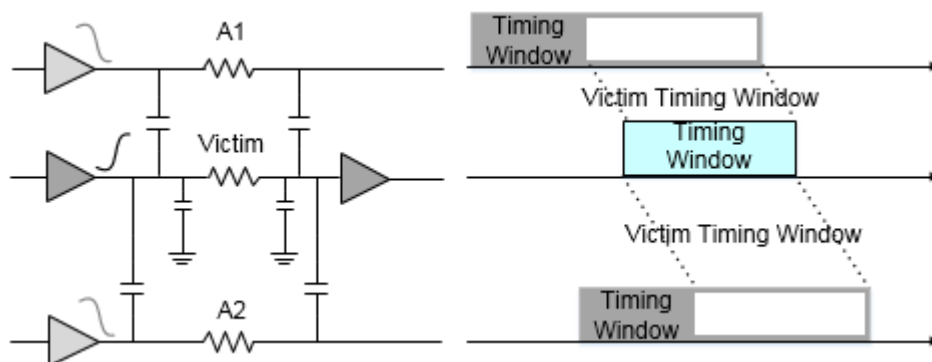
Figure 4-24 Timing-Aware Edge Alignment Mode - Illustration 1
