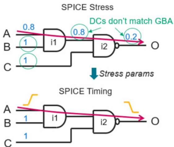
Figure 4-103 Method 1 (Stress and Timing correlation)
