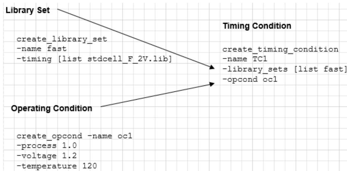
Figure 5-3 Define timing conditions
