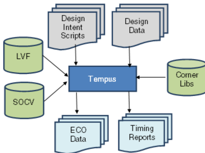
Figure 4-73 SOCV Data Flow
