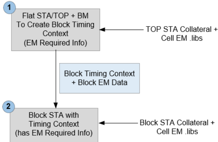
Figure 4-122 Cell EM Context-Based Flow
