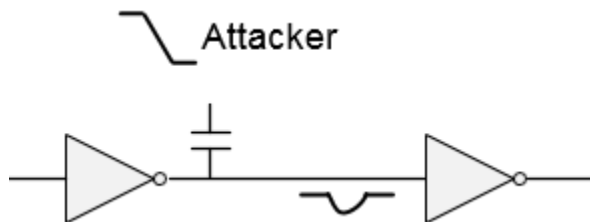
Figure 4-54 VL, VH, VLU, and VHO glitch waveforms
