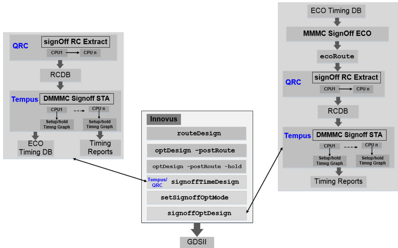
Figure 8-4 Signoff Timing Optimization Flow
