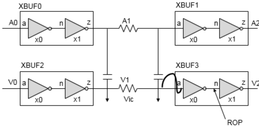
Figure 4-48 ROP (Receiver Output Peak) for multi-stage cell
