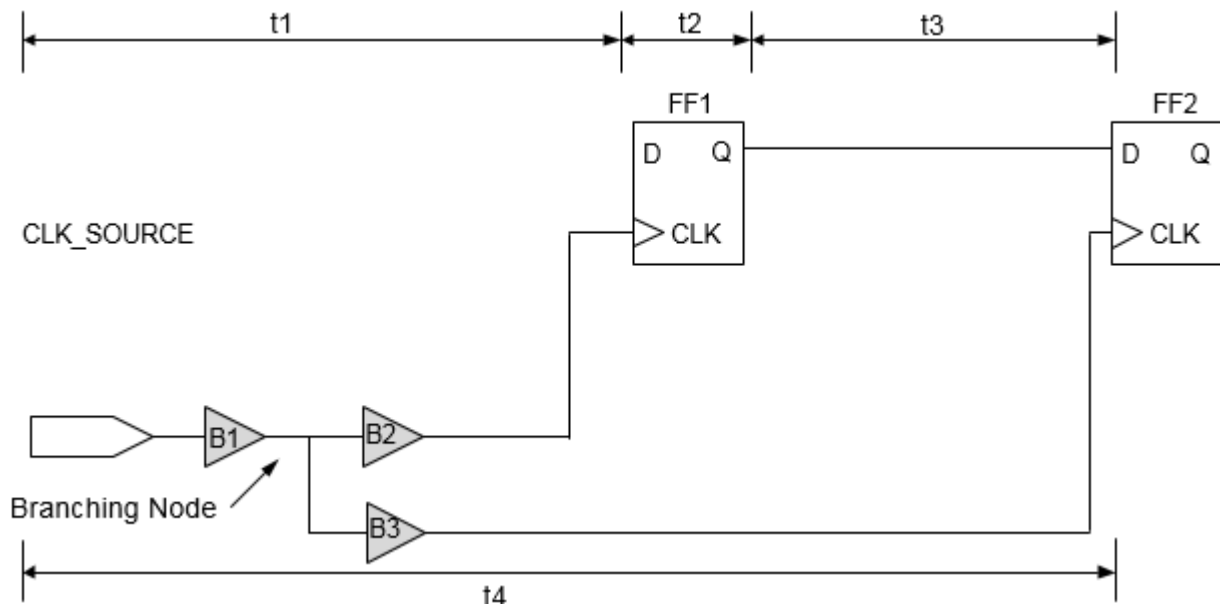
Figure 4-66 Signal Path
