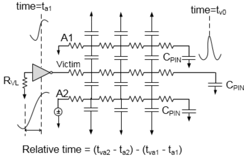
Figure 4-40 Aligning Attackers to Have Worst Impact at Victim at Same Time
