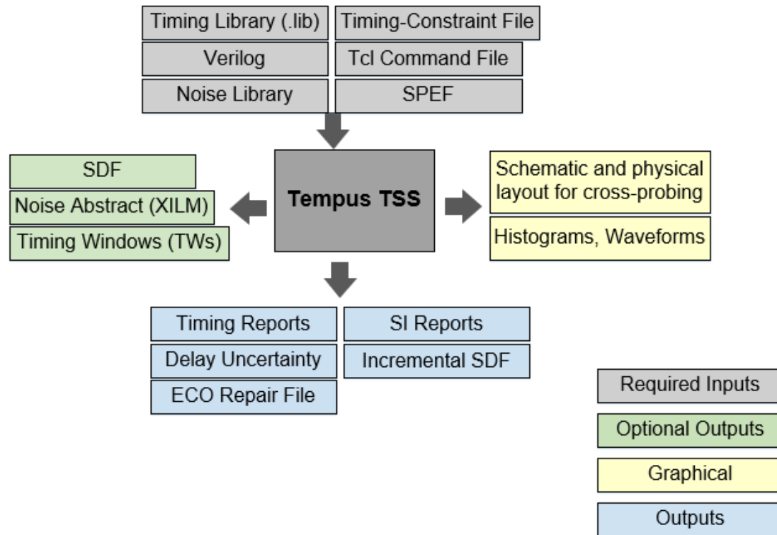
Figure 4-3 Inputs and Outputs required for Base and SI Analysis
