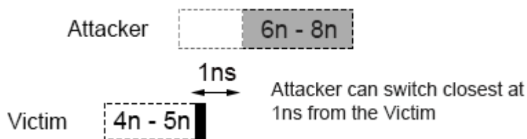
Figure 4-18 Timing window of Attacker and Victim not Overlapping
