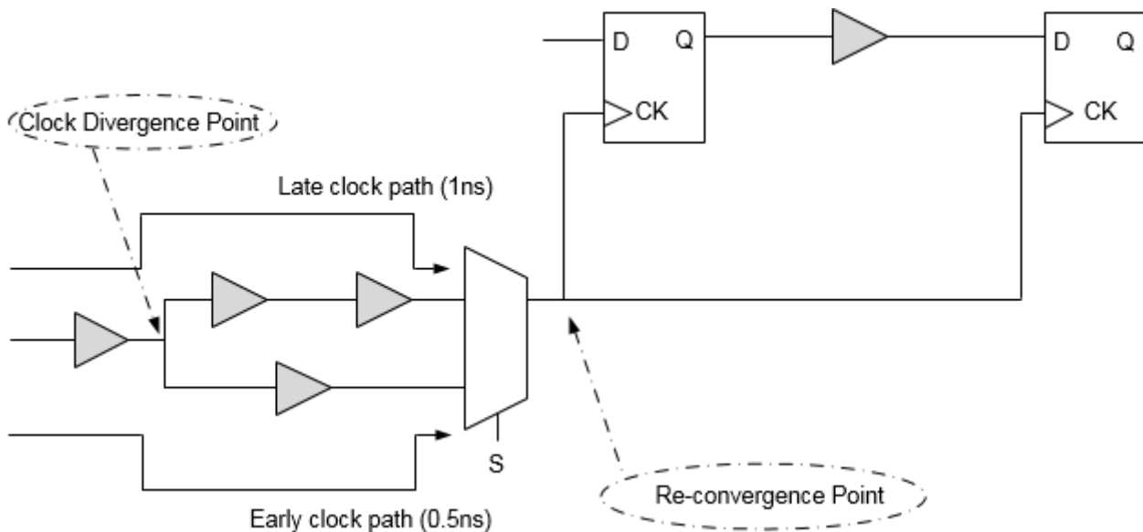
Figure 4-67 Illustration of Clock Re-convergence
