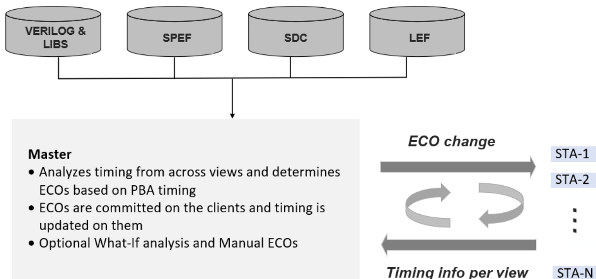
Figure 1-5 Tempus Paradime Flow Licensing in CMMM Mode
