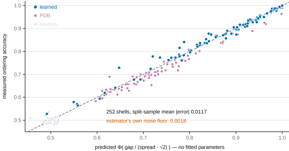
Figure 3: Predicted against measured ordering accuracy; the dashed line is y = x . Pattern databases sit slightly below it, which is the cost of their discreteness — the one place the normal approximation is visibly imperfect.
