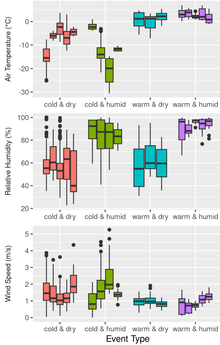
Figure 6: Boxplots of showing the distribution of meteorological measurements of air temperature, relative humidity, and wind speed over each of the seventeen selected ablation events. Air temperature, relative humidity, and wind speed were measured at FT station. Note: the rectangle vertical extent represents the interquartile range (25 th to 75 th percentile), the horizontal line within each box indicates the median, and the whiskers extend to 1.5 times the interquartile range. Circular points beyond the whiskers represent outliers.
