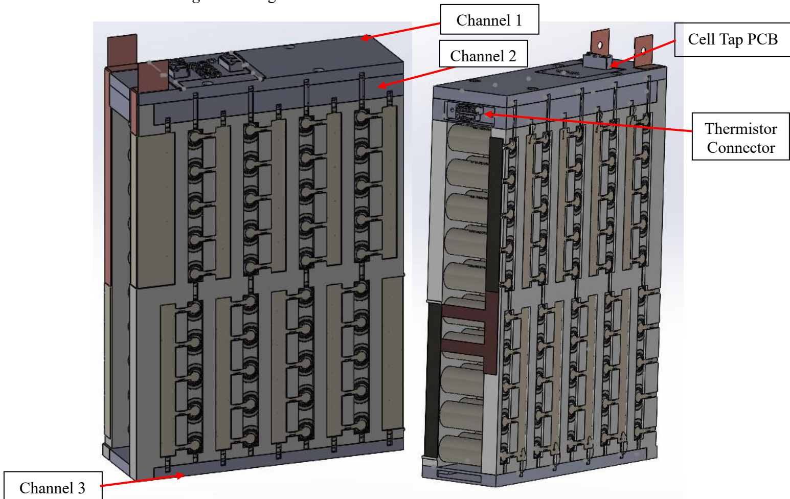
Figure 92: 9x10 Accumulator Segment
