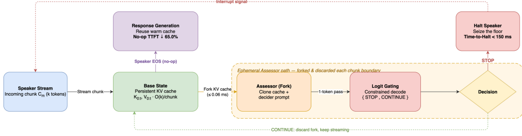
Figure 1: Dual-State KV-Forking . Speaker chunks update the Base cache ( O(k)/\text{chunk} ). At each boundary the cache is forked ( \leq 0.06 ms) into an Assessor emitting one gated STOP/CONTINUE token. CONTINUE discards the fork; STOP halts the speaker in sub-150 ms; on natural completion the warm cache generates the response immediately.
