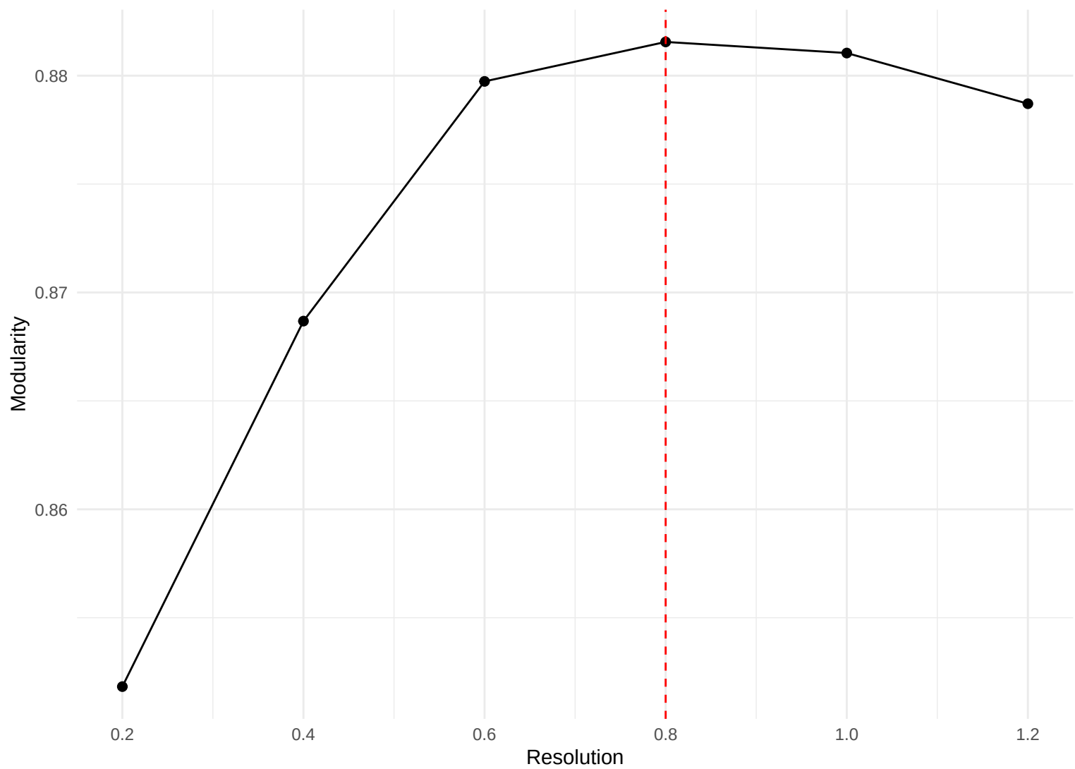
Modularity vs Resolution
