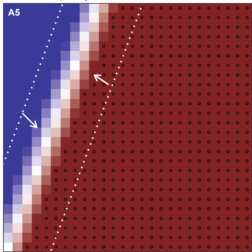
Lower inequality
