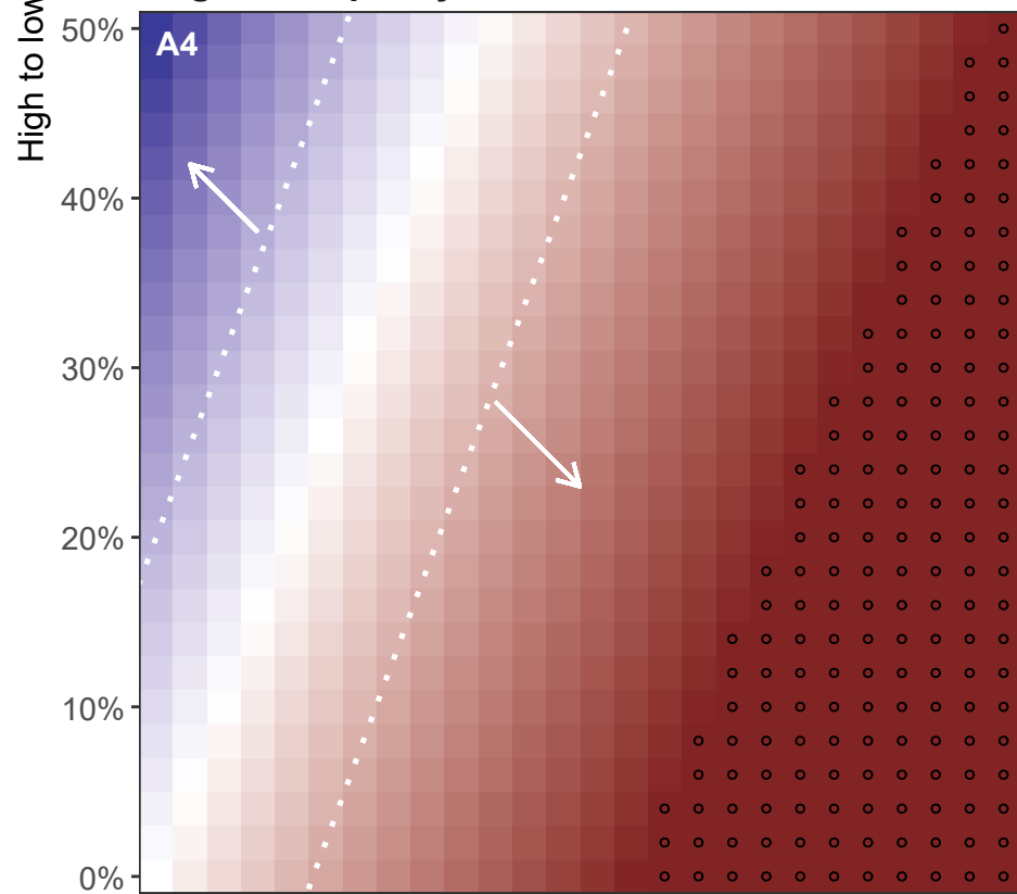
Higher inequality
