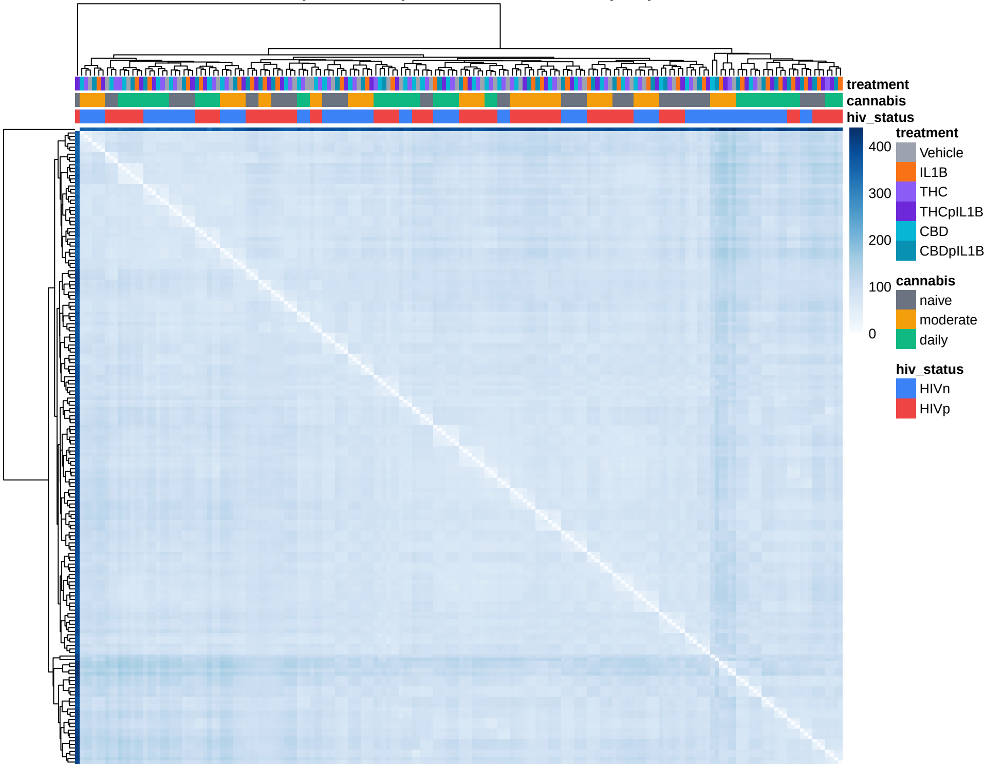
Sample-to-sample Euclidean distances (VST)
