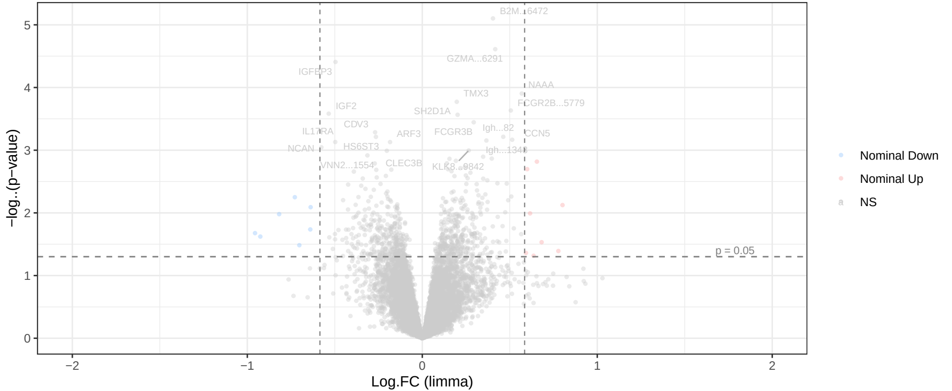
Daily vs Naive | Proteomics FDR < 0.05: n = 0 | Nominal p < 0.05: n = 22
