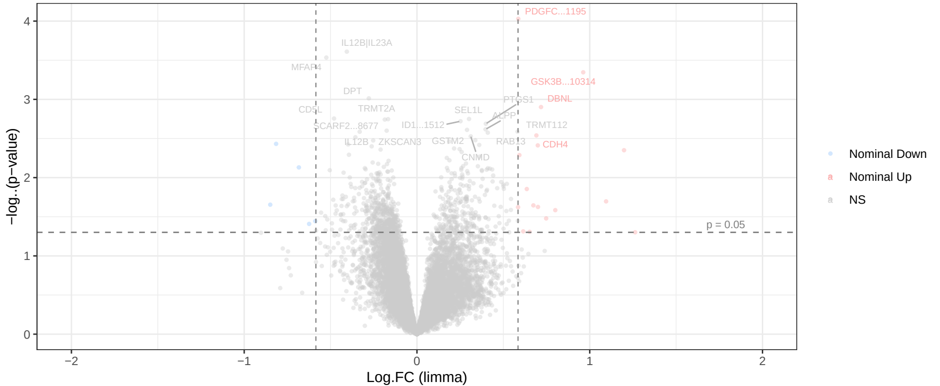
Moderate vs Naive | Proteomics FDR < 0.05: n = 0 | Nominal p < 0.05: n = 7
