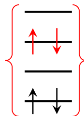
Doubly Excited States
