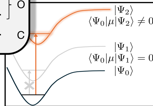
Transition Dipole Moments
