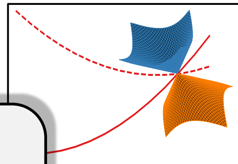
Conical Intersections
