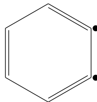
Diradicals
