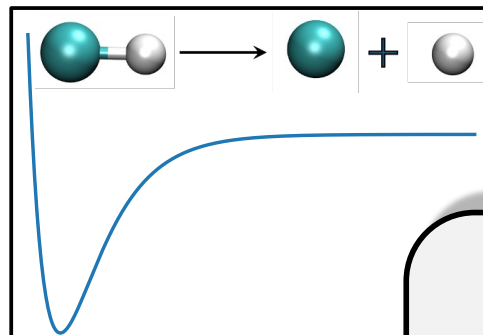
Bond Breaking
