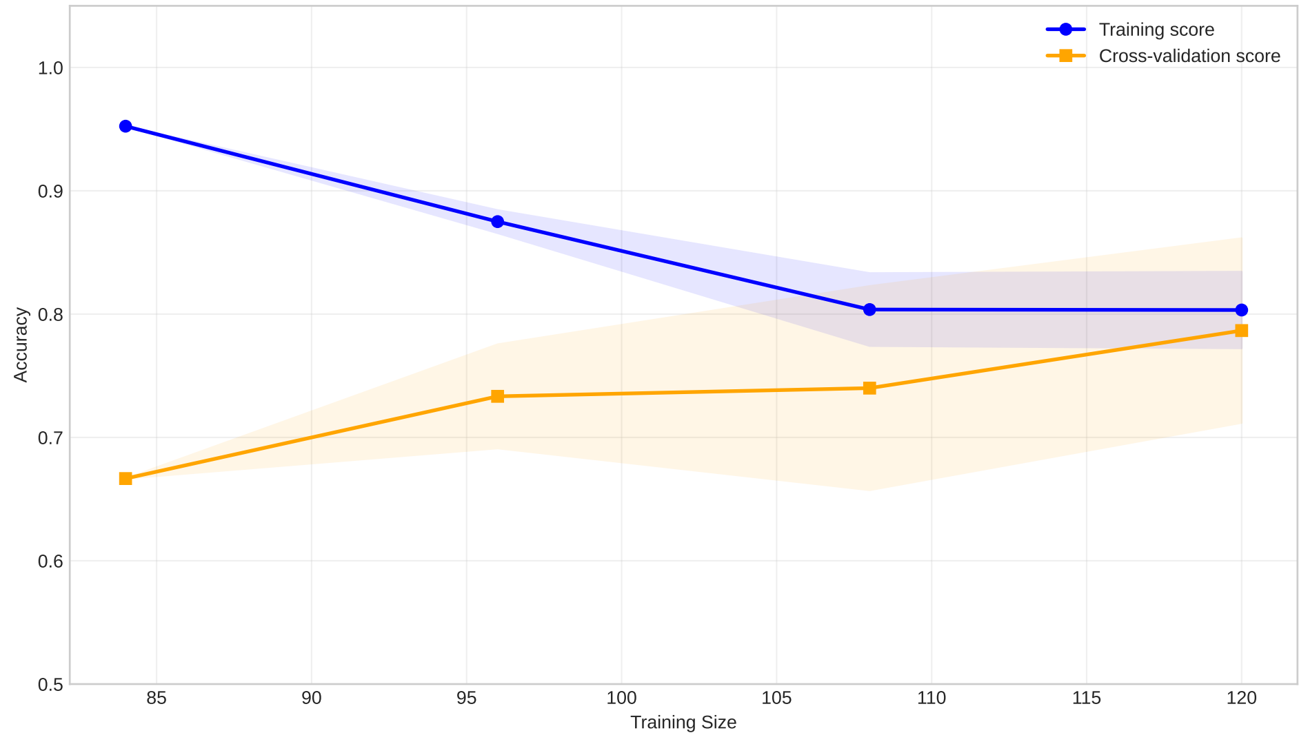
Learning Curve: Logistic Regression
