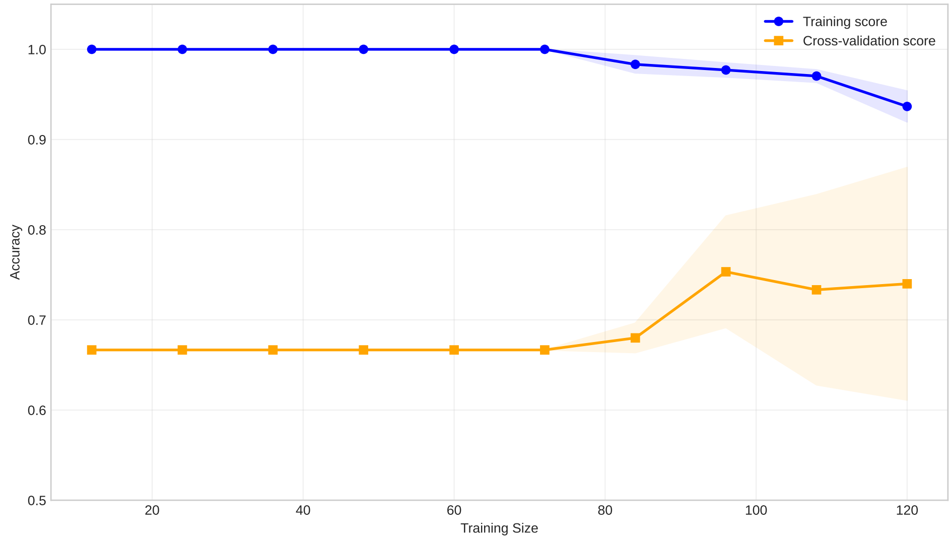
Learning Curve: Random Forest
