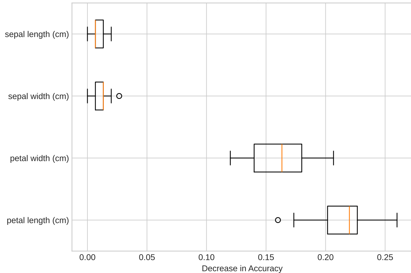
Permutation Importance
