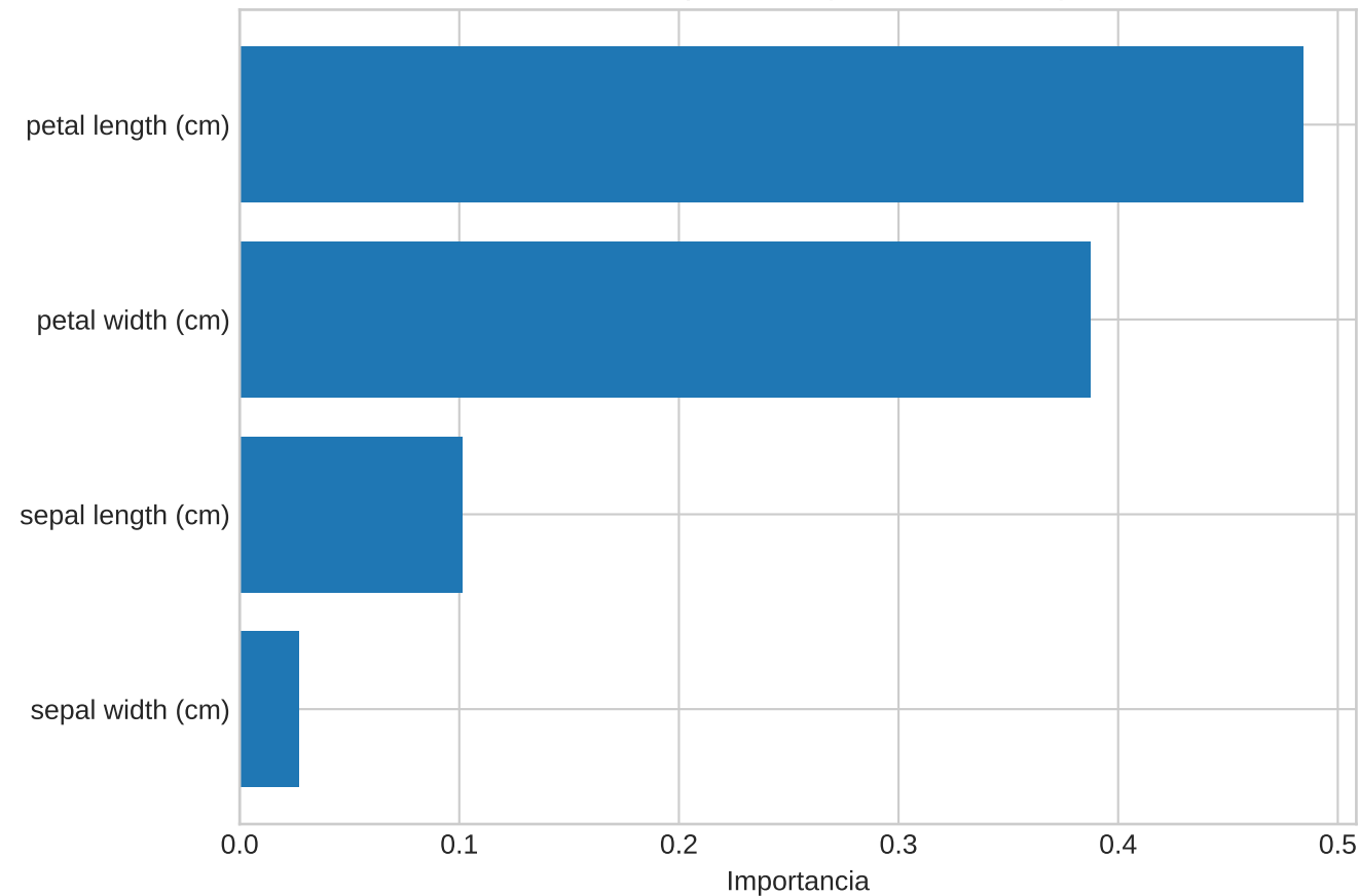
Feature Importance (Random Forest)
