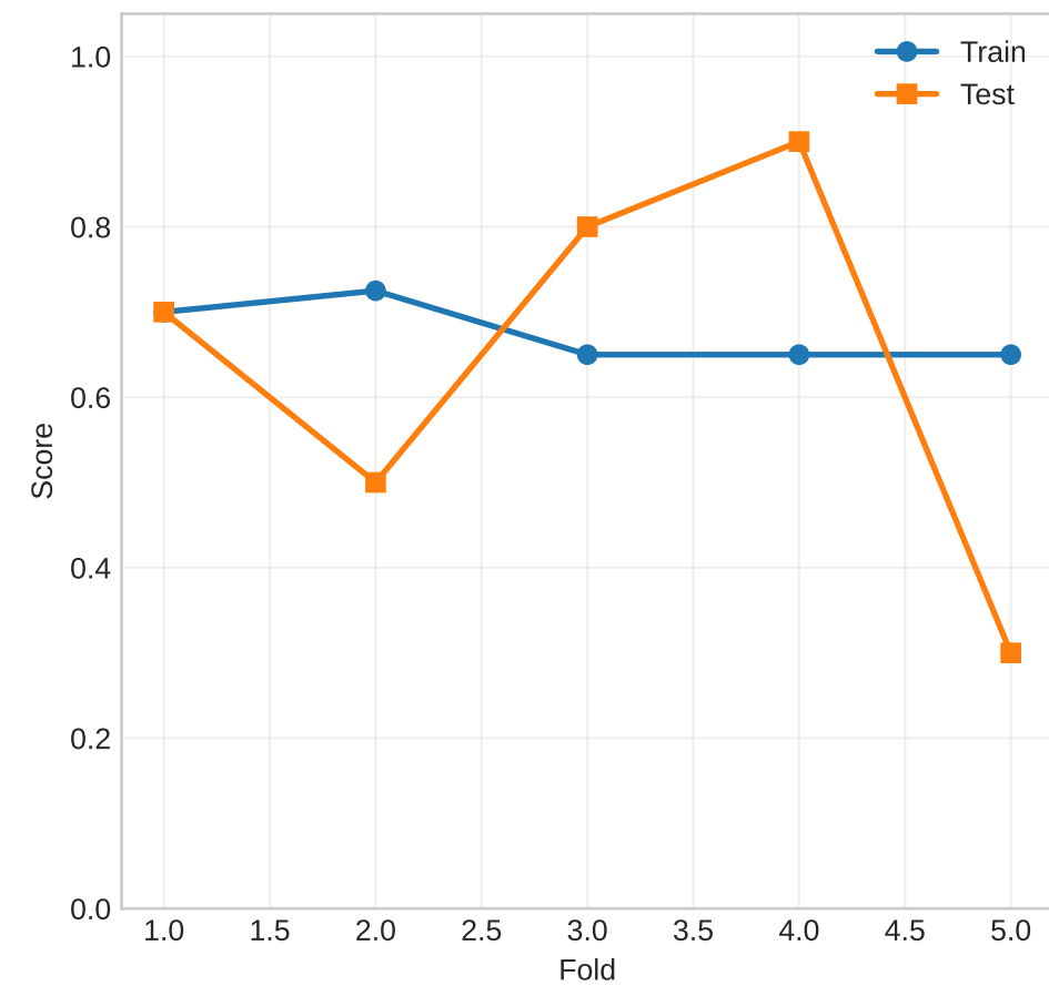
RECALL
