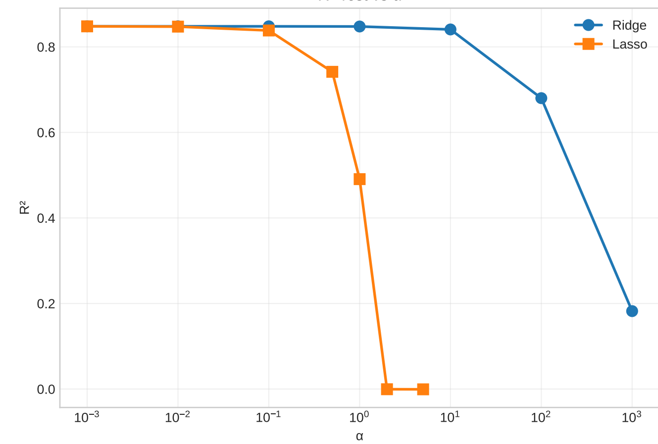
R^2 Test vs \alpha
