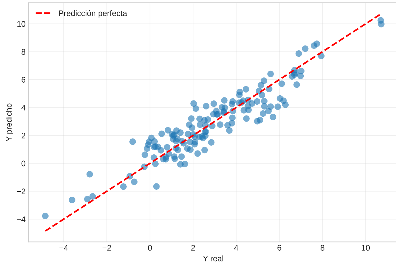
OLS - Entrenamiento ( R^2=0.862 )
