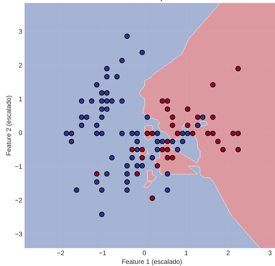
k=15, Accuracy=0.711
