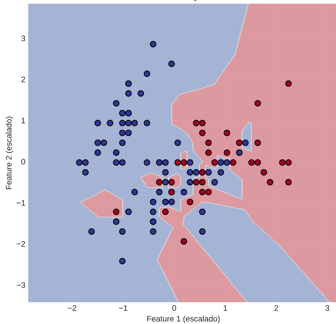
k=10, Accuracy=0.756
