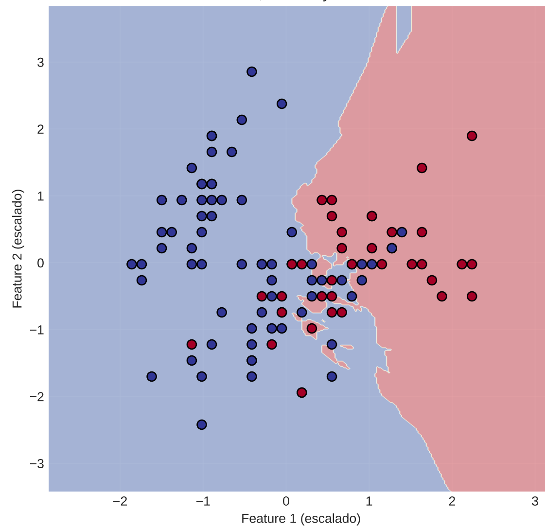
k=15, Accuracy=0.711
