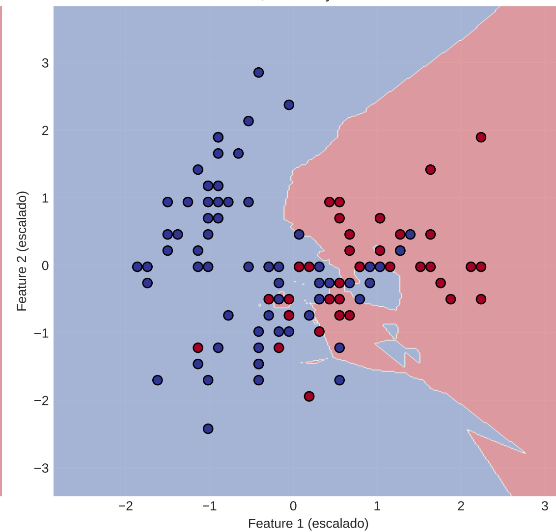
k=20, Accuracy=0.756
