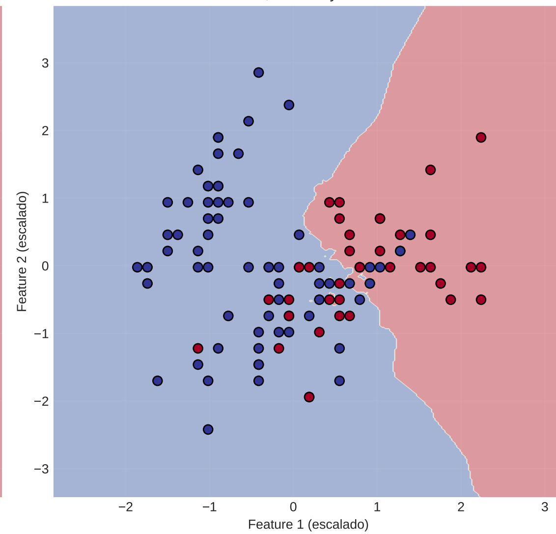
k=20, Accuracy=0.756
