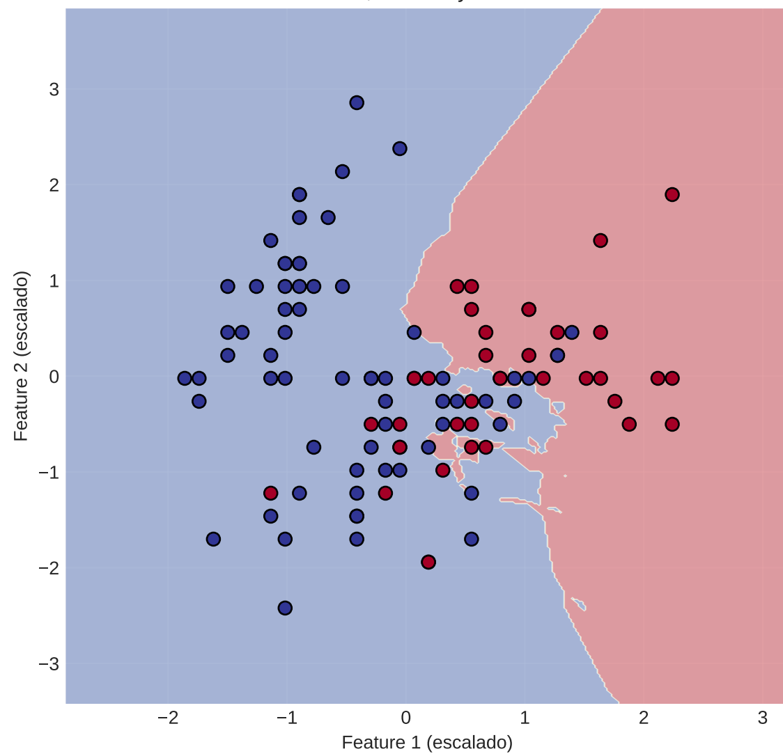
k=10, Accuracy=0.756
