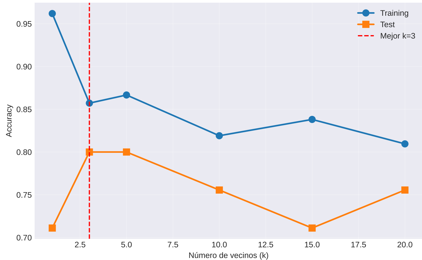
Accuracy vs K
