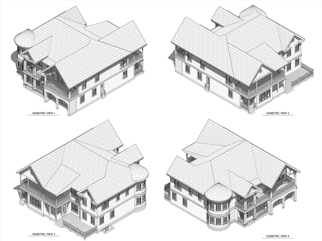
ISOMETRIC VIEWS
