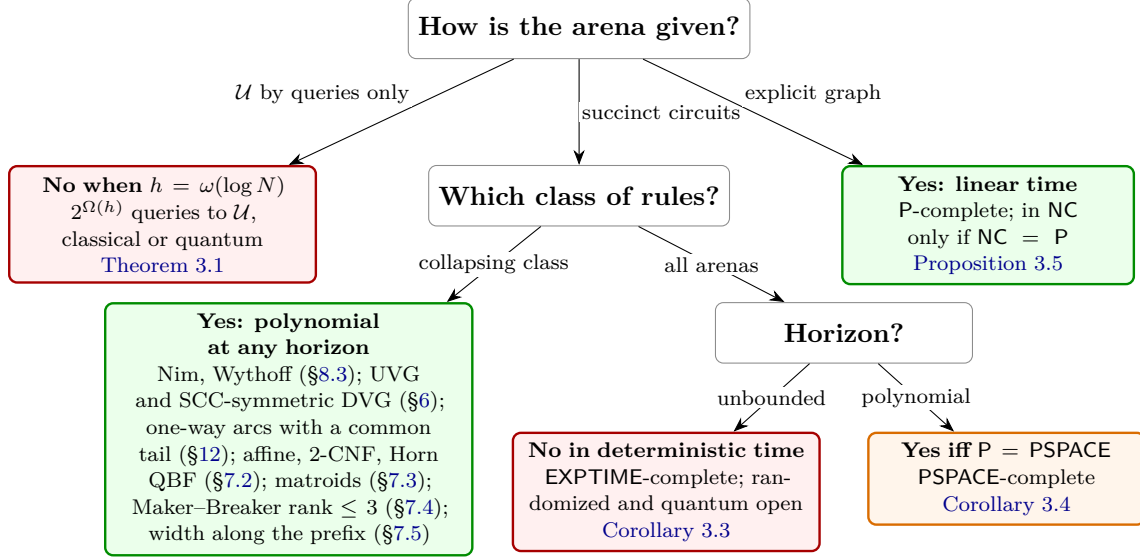
FIGURE 1. Verdicts on the existence of a polynomial-time invariant \Phi with \mathcal{V} = f \circ \Phi , by representation, rule class and horizon. Each “no” verdict is for the class of all arenas in the model its box names; the small print names the proof.
