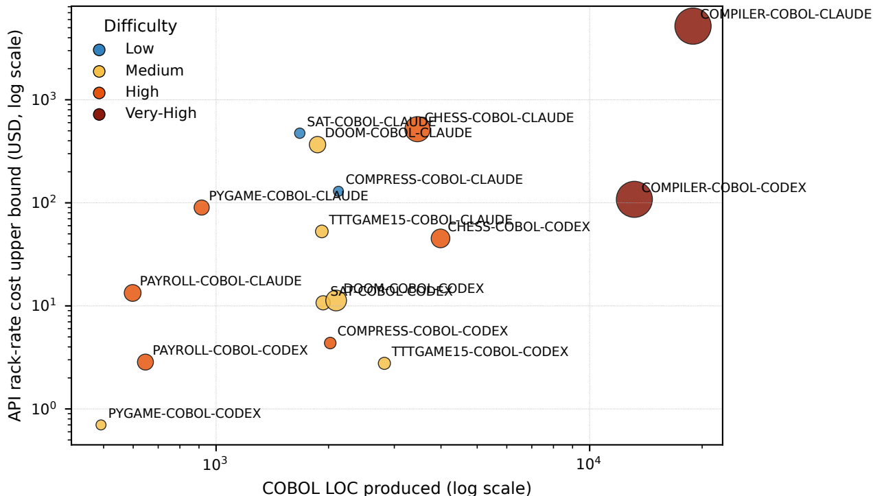
Compute cost vs COBOL output (bubble \propto user-prompt count)
