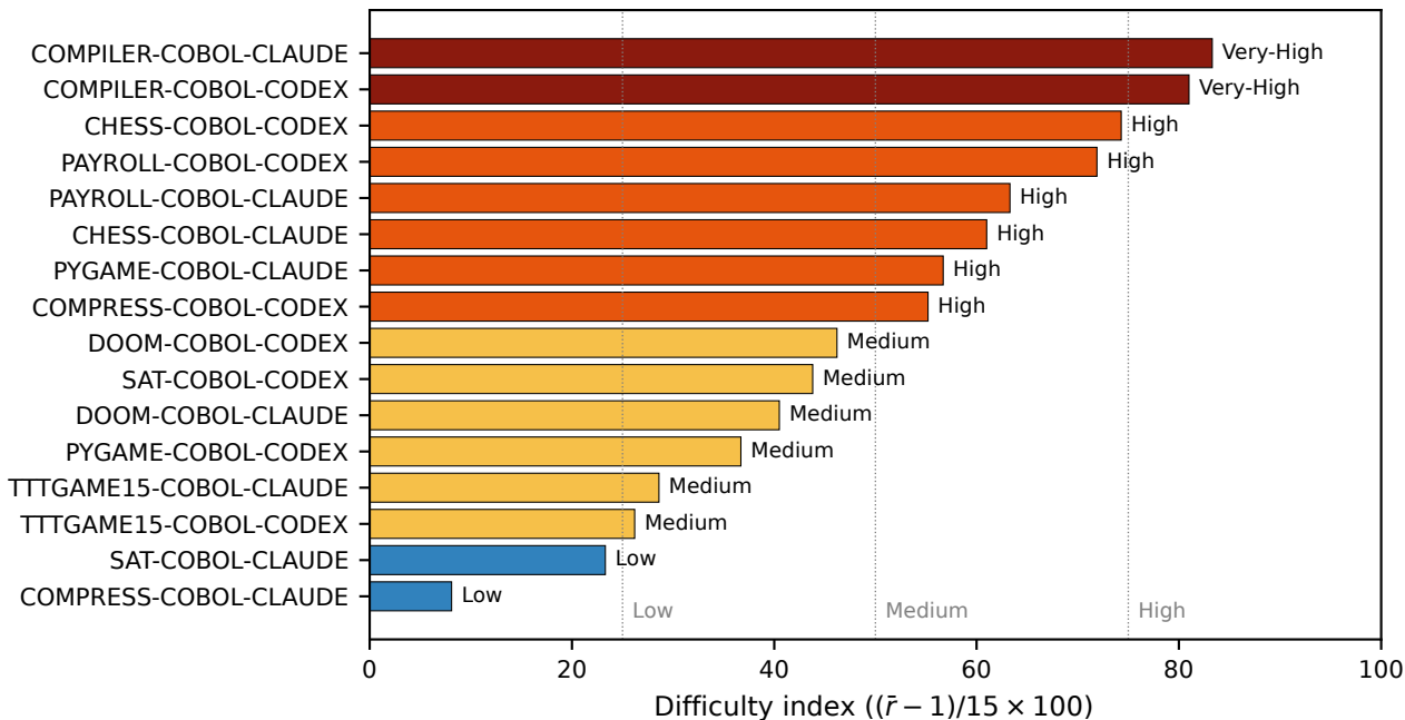
Per-project difficulty index (low = easier, high = harder)
