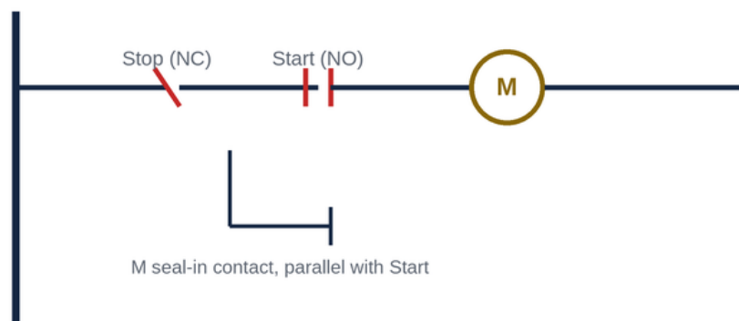
Figure FC-27.1 — A basic three-wire start-stop control rung with seal-in contact.
