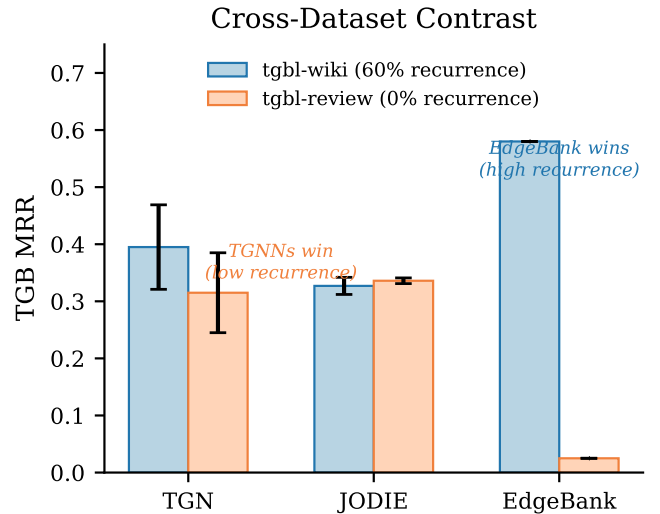
Figure 4: Cross-dataset contrast. On high-recurrence wiki, EdgeBank dominates; on low-recurrence review, TGNNs dominate. The crossover is consistent with edge-recurrence rate as the determining factor.
