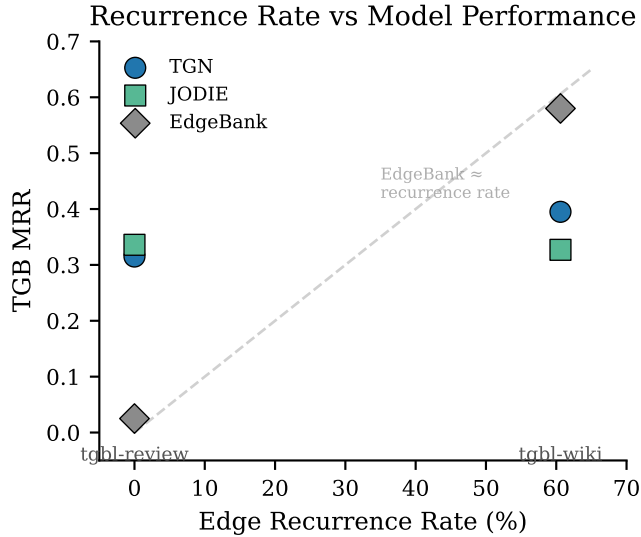
Figure 5: Model performance vs. edge recurrence rate. EdgeBank’s MRR closely tracks recurrence (dashed line); learned models remain stable, dominating in the low-recurrence regime.
