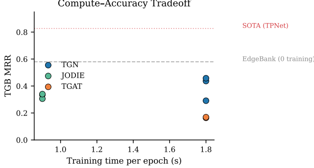
Figure 3: Compute-accuracy tradeoff. EdgeBank (dashed gray) dominates with zero training time. No TGN reaches the EdgeBank line.
