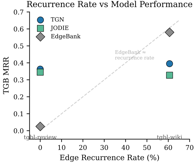
Figure 5: Model performance vs. edge recurrence rate. EdgeBank’s MRR closely tracks recurrence (dashed line); learned models remain stable, dominating in the low-recurrence regime.
