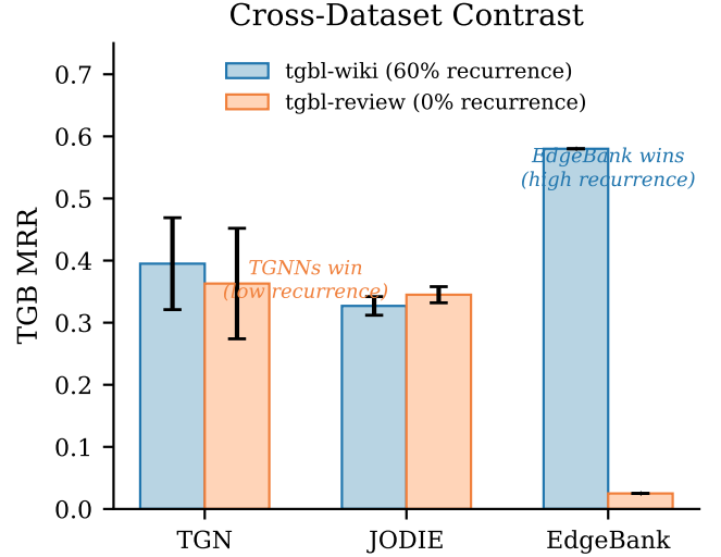
Figure 4: Cross-dataset contrast. On high-recurrence wiki, EdgeBank dominates; on low-recurrence review, TGNs dominate. The crossover is consistent with edge-recurrence rate as the determining factor.
