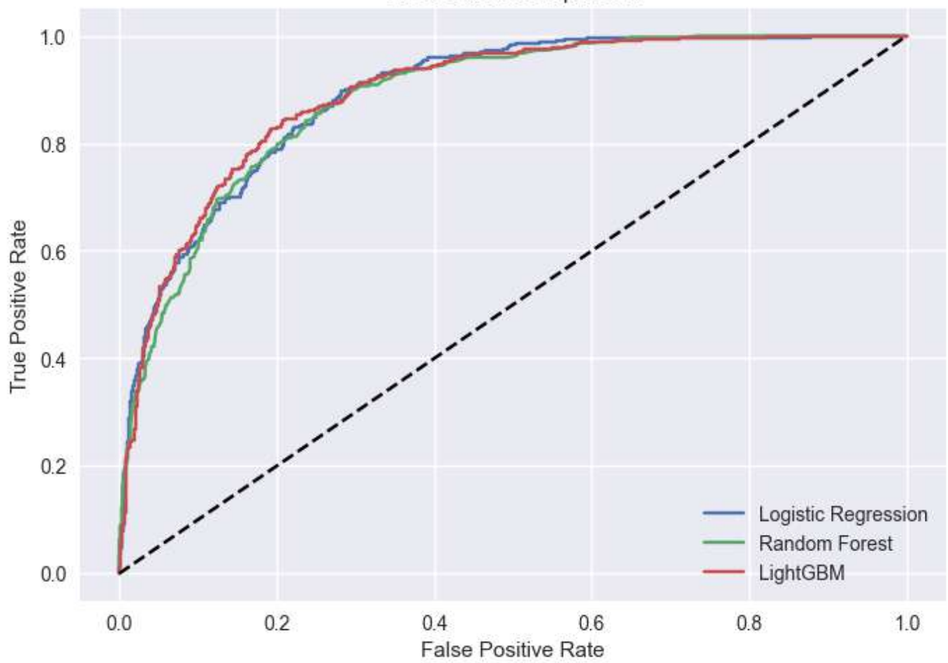
ROC Curve Comparison
