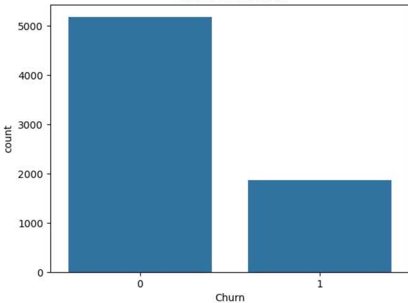
Churn Distribution
