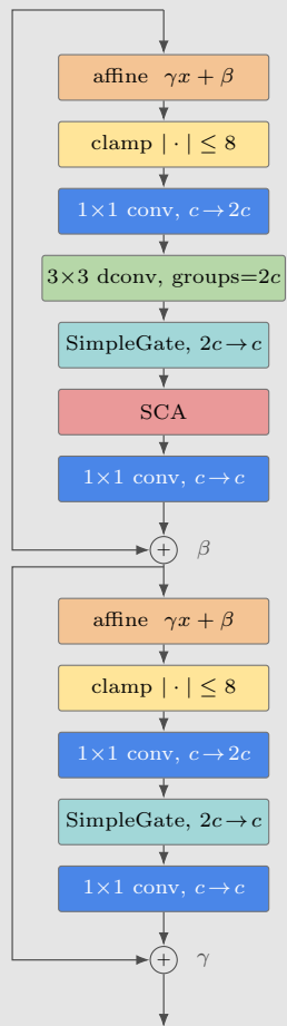
(b) full-resolution block enc0, dec3 ( c = 16 )
