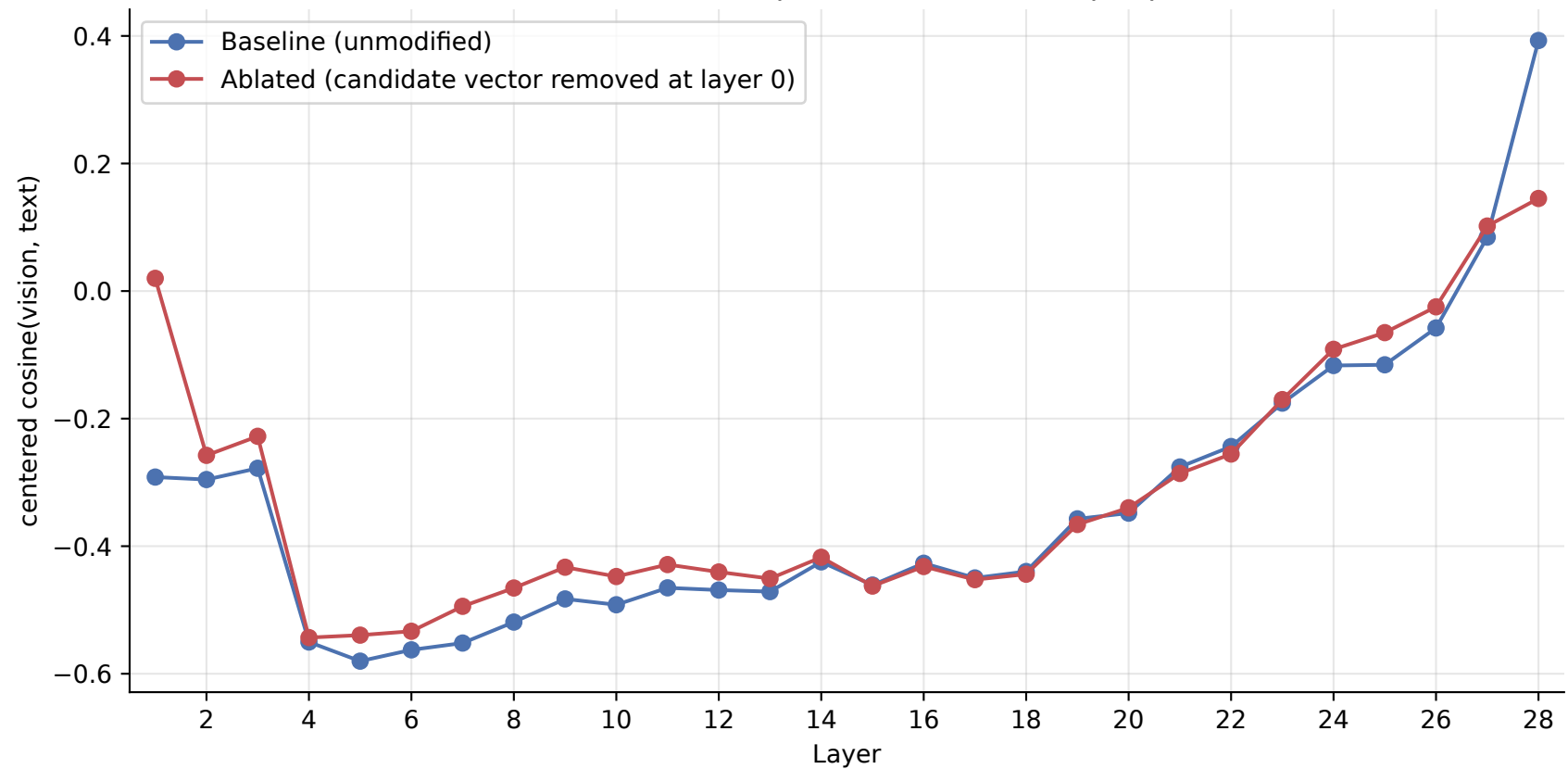
Vision-text representational similarity across layers Qwen2-VL-7B-Instruct, 500 pairs each, centered per-pair cosines
